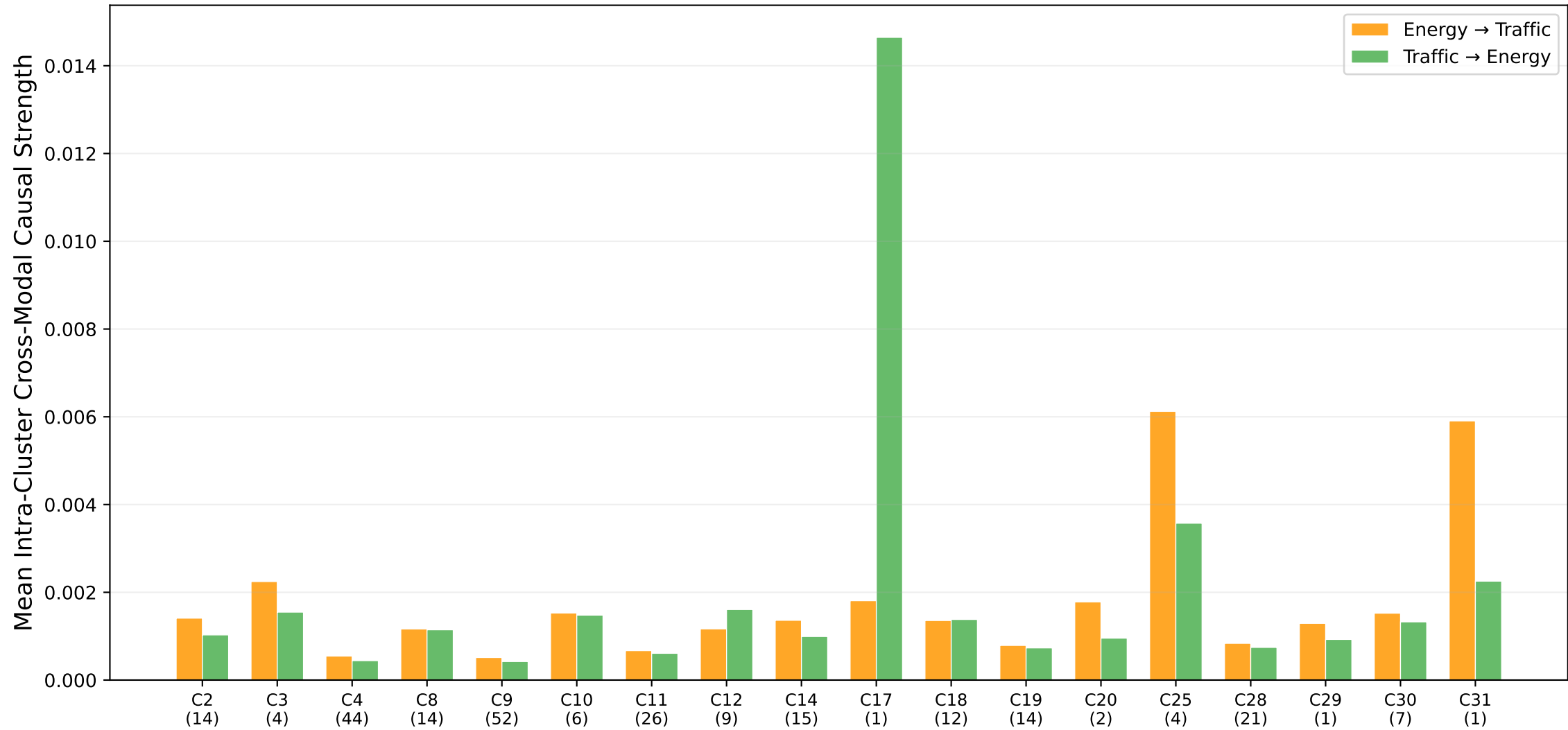
(b) Causal Asymmetry per Cluster: Which Direction Dominates?
