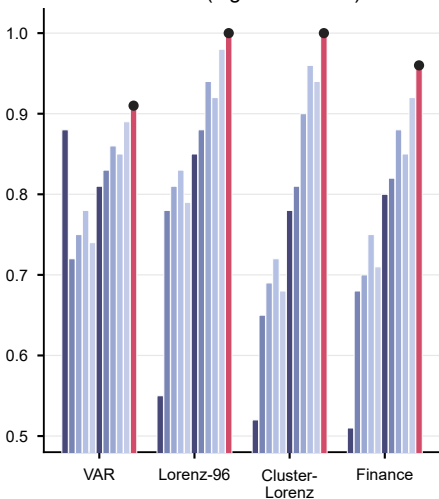
AUROC (higher is better)
