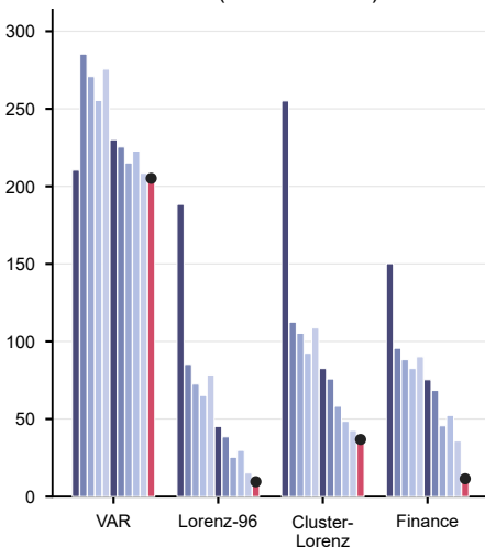
SHD (lower is better)
