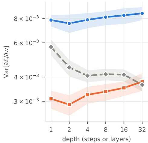
(a) line detection, 5 qubits
