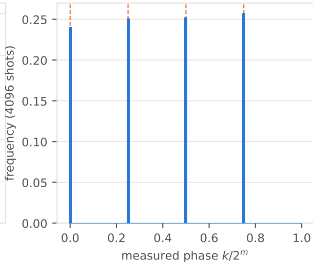
(b) phase estimation on U_a , m = 8
