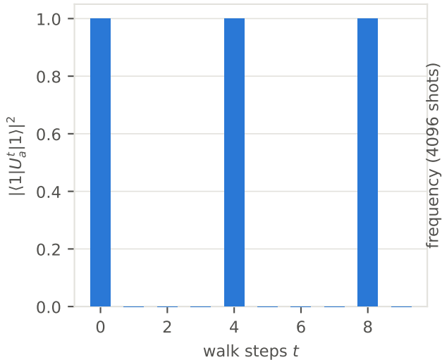
(a) revival of the walk, N = 15 , a = 7 , r = 4
