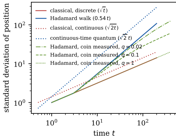
(c) spread against time
