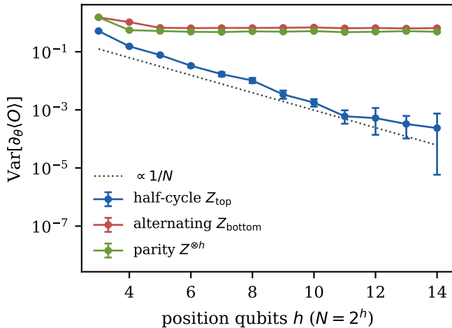
(a) walk-time ansatz e^{-itA} , t \sim U[0, 8]
