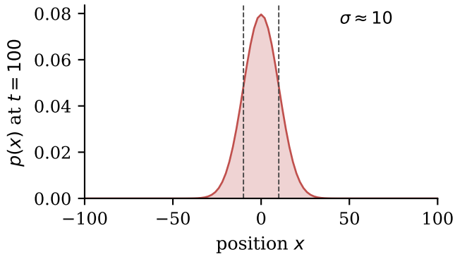
Classical random walk
