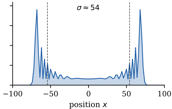
Hadamard quantum walk
