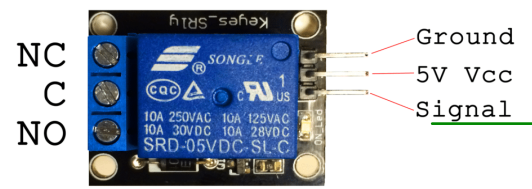
5V Relay Terminals and Pins
