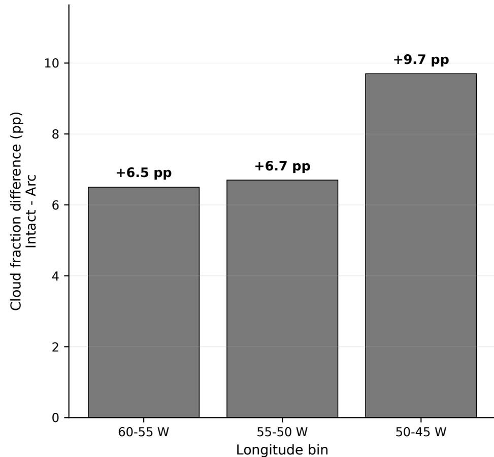
(b) Cloud cover loss in deforested arc
