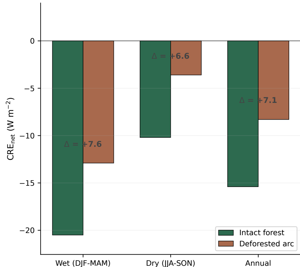
(a) CRE net : intact forest vs deforested arc
