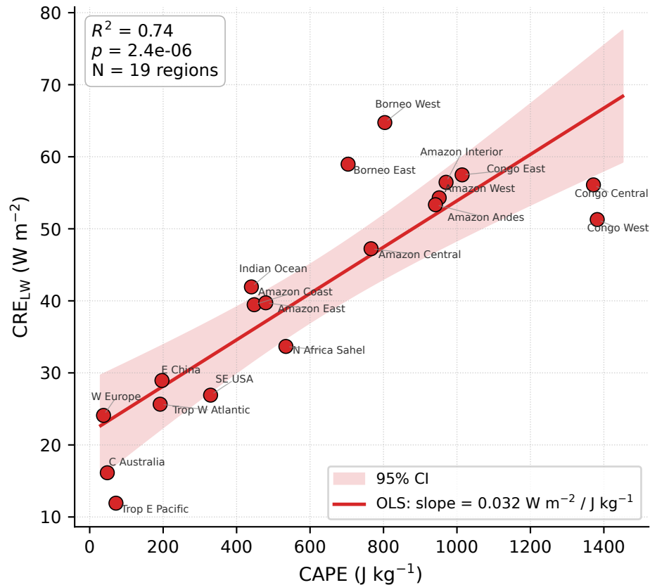
(a) CRE LW scales with CAPE
