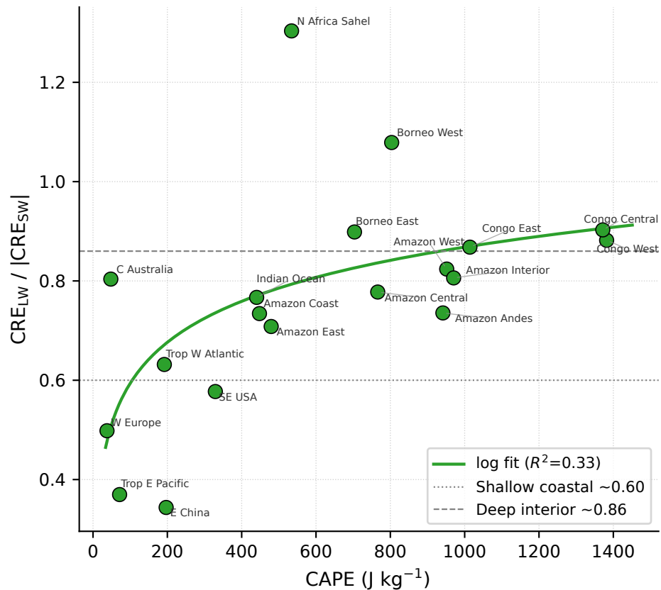
(b) Convective-depth regulation of SW/LW partition
