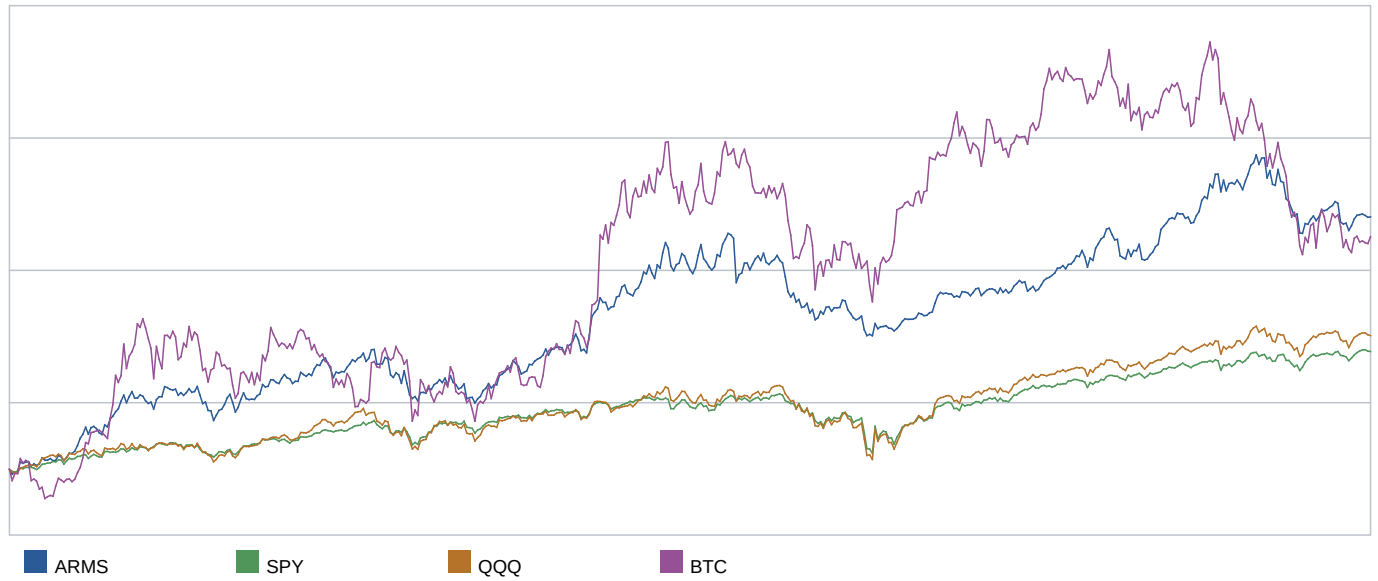
Growth of $100
