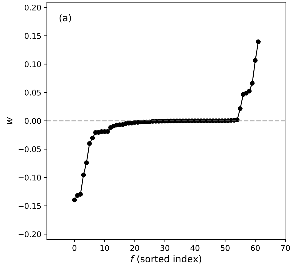
Tg_fitted
