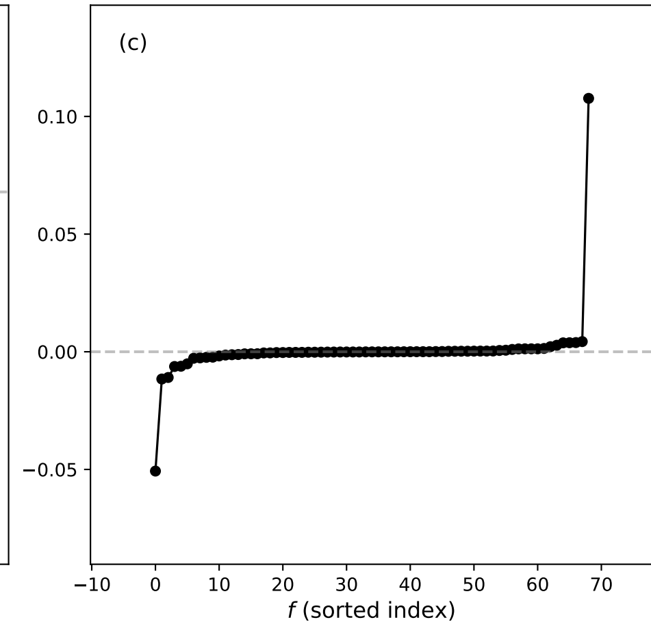
log_eta_inf_fitted
