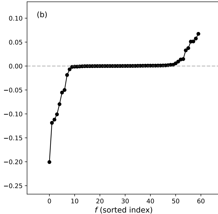
m_fitted
