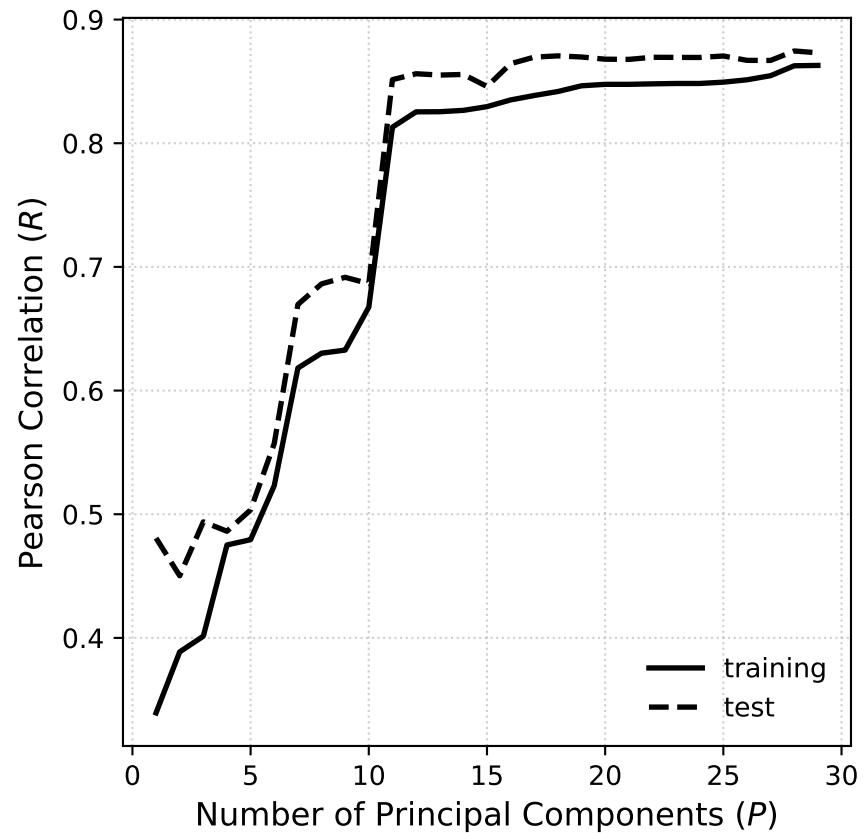
PCR Performance vs Components: m_fitted
