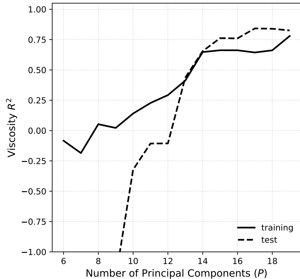
Global Viscosity Predictive Performance vs P (Classical PCR)
