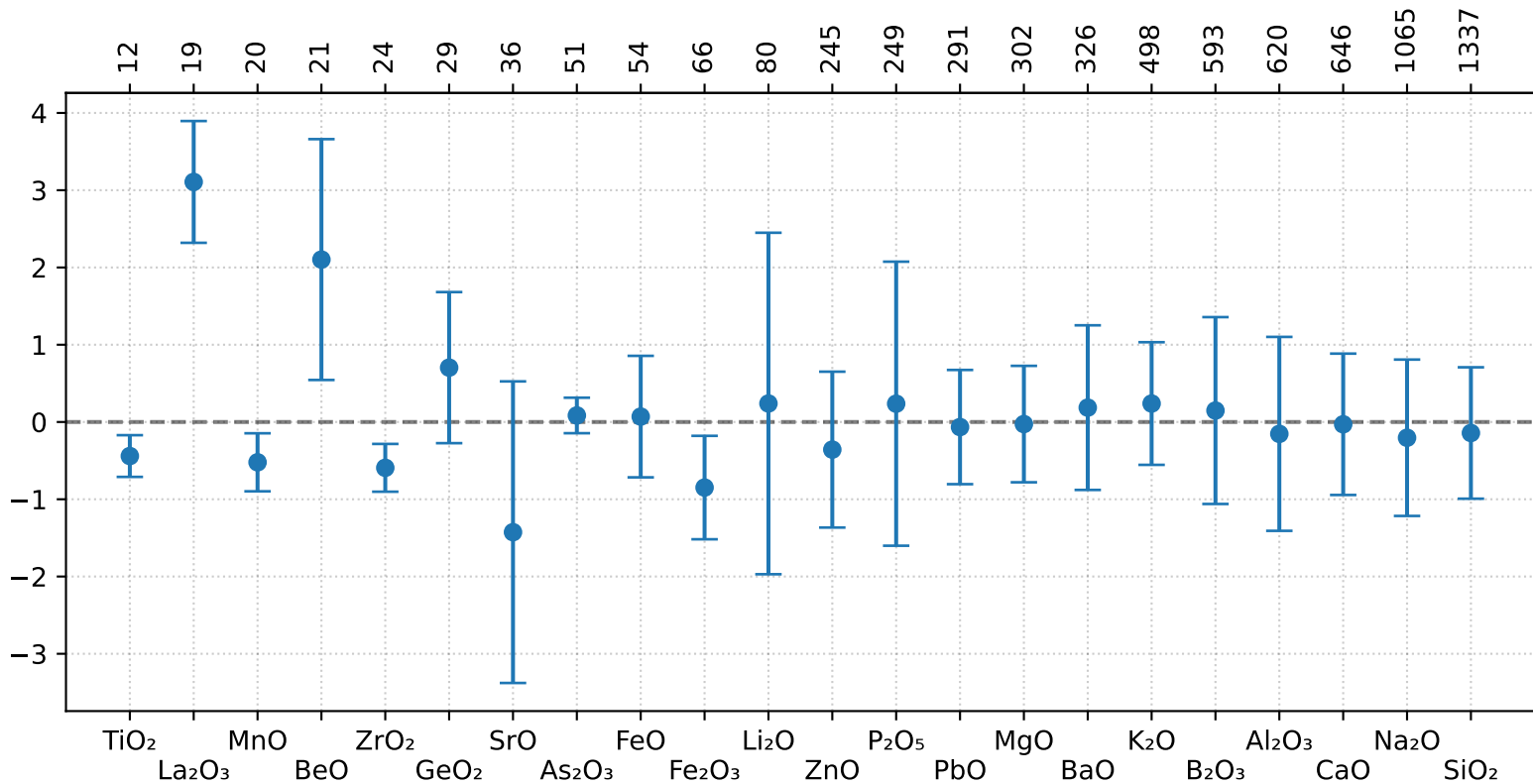
Viscosity Prediction residual ( \log_{10} \eta )
