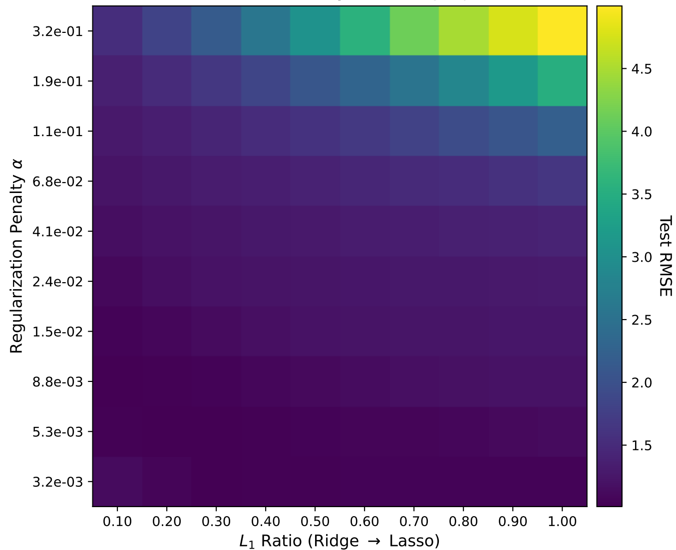
Global Viscosity RMSE ( \log_{10} \eta )
