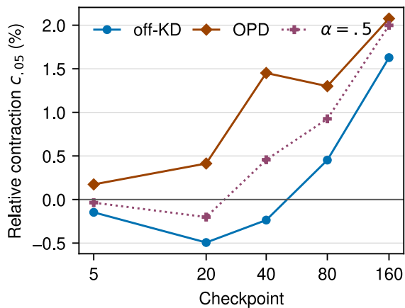
(c) frozenSelf0-KD minus OPD margin
