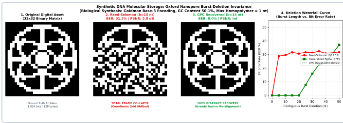
Fig. 1: 32 \times 32 DNA image recovery under 15 \text{ nt} Nanopore burst deletion.
