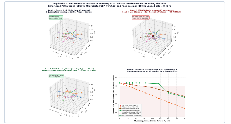
Fig. 2: 8-quadcopter 3D trajectories under 60 \text{ ms} RF jamming burst.
