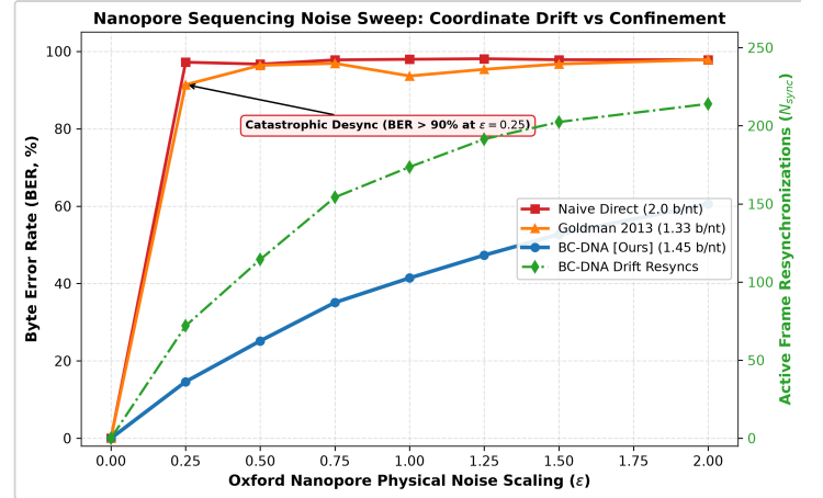
Figure 2. Empirical Performance Under Oxford Nanopore Sequencing Noise Sweep. As physical noise scaling \epsilon increases from 0.0 to 2.0, Naive Direct and Goldman 2013 collapse immediately into total coordinate desynchronization ( extBER > 91.4\% at just \epsilon = 0.25 ). In contrast, BC-DNA actively engages its Bounded-Slip Markers (triggering over 200 frame resynchronizations), confining errors to local blocks and exhibiting graceful degradation.
