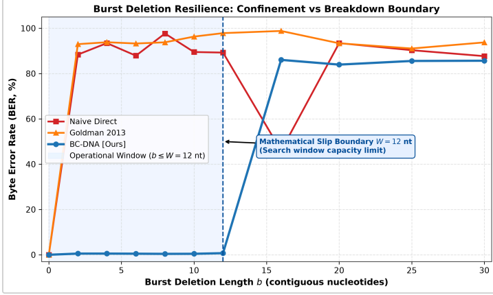
Figure 3. Localized Burst Deletion Stress Test & Breakdown Boundary. Contiguous burst deletion sweep b \in [0, 30] \text{extnt} on a 1,920-byte payload. For all bursts within the search window b \leq W = 12 \text{extnt} , BC-DNA confines corruption strictly to the affected block, maintaining global \text{extBER} \leq 0.7\% . When burst length exceeds the search window ( b > 12 ), the marker slips beyond the search radius, correctly exposing the algorithm's operational breakdown boundary (Math input error). Baselines collapse to \text{extBER} > 88\% for any b \geq 2 \text{extnt} .
