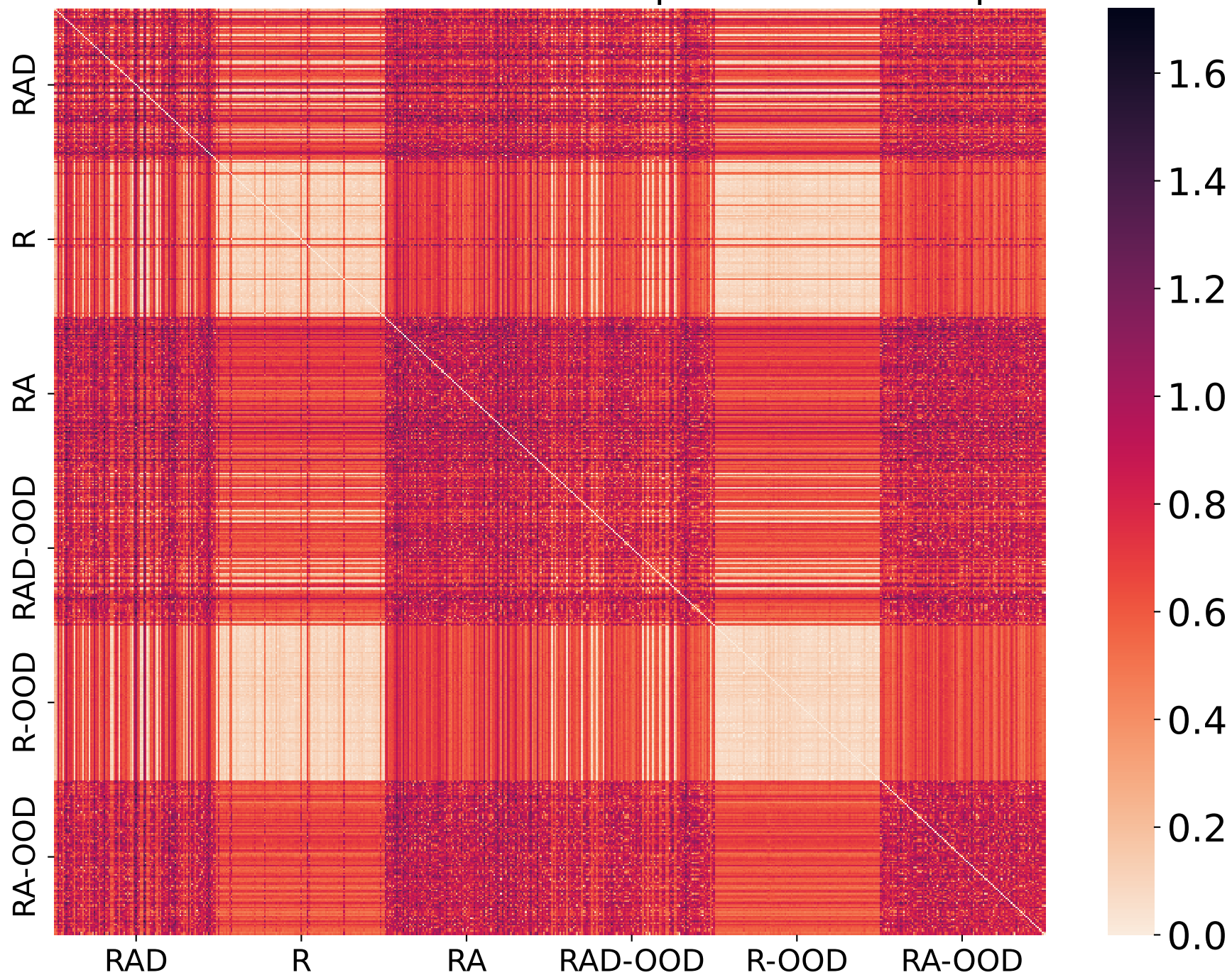
Normalized L2 Distance Heatmap of Encoder Outputs
