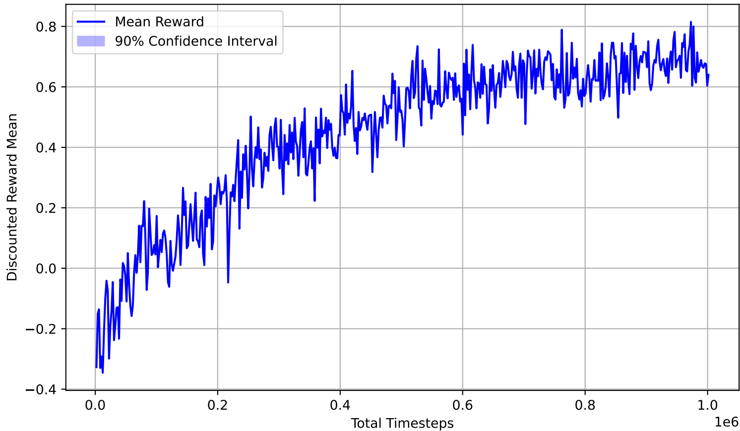
Learning Curve with 90% Confidence Interval
