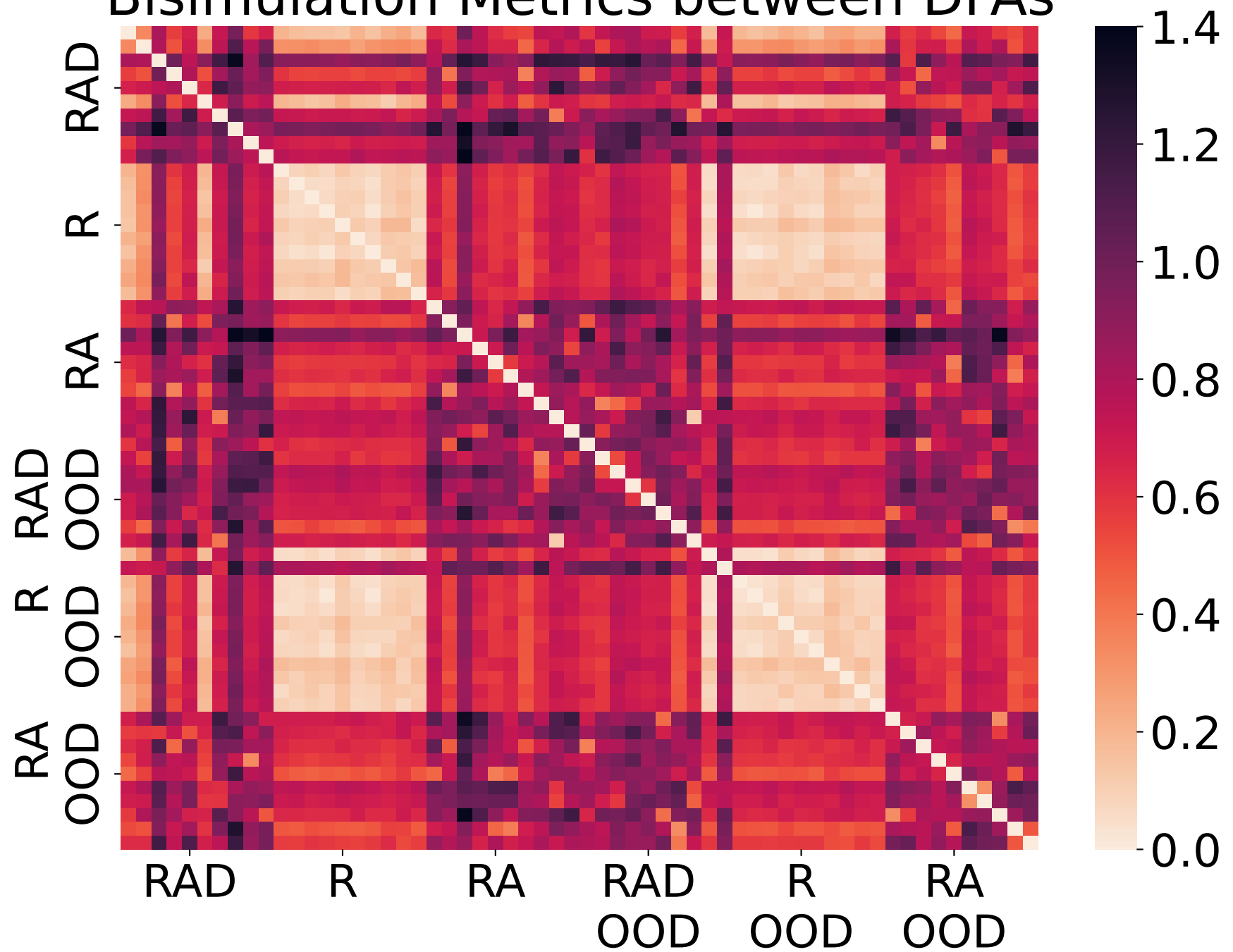
Bisimulation Metrics between DFAs
