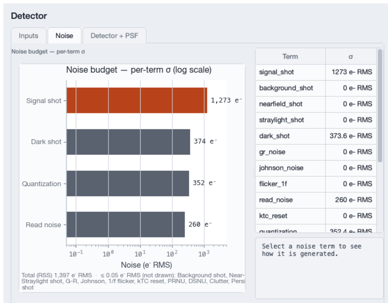
Figure 2.7: Detector workspace, Noise tab — the per-term noise budget on a log axis beside the same terms as a table.
