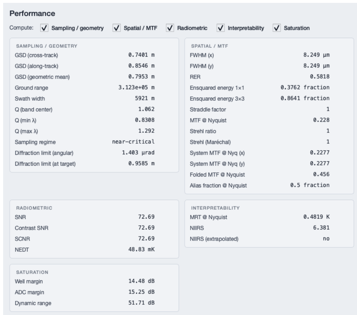
Figure 6.3: Performance workspace at 30° off nadir.
