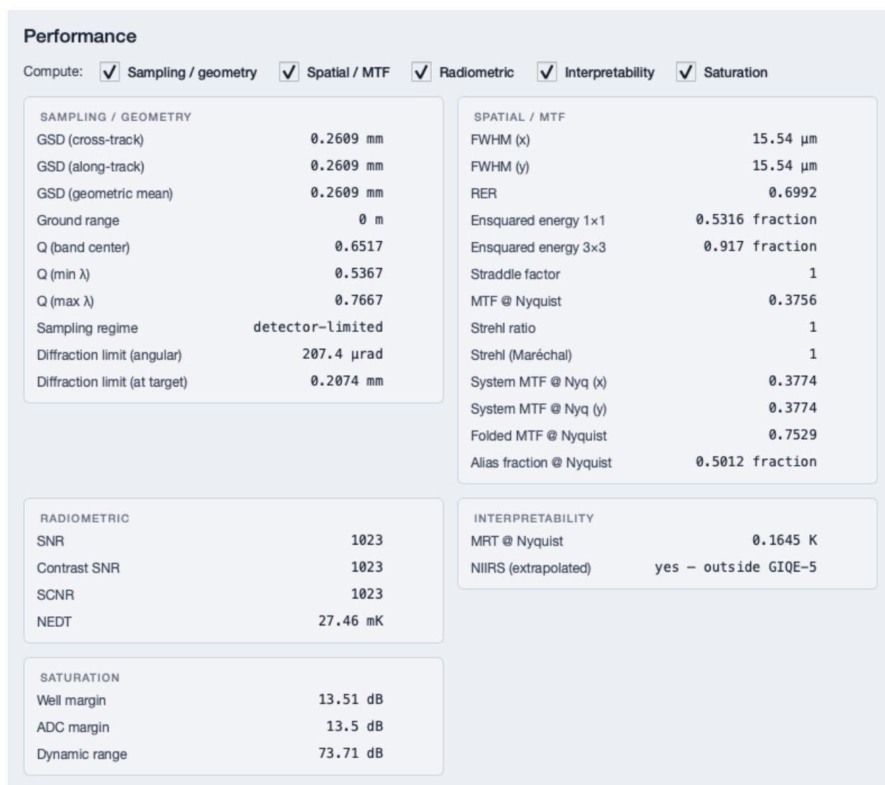
Figure 5.4: Performance workspace on the InSb bench branch.
