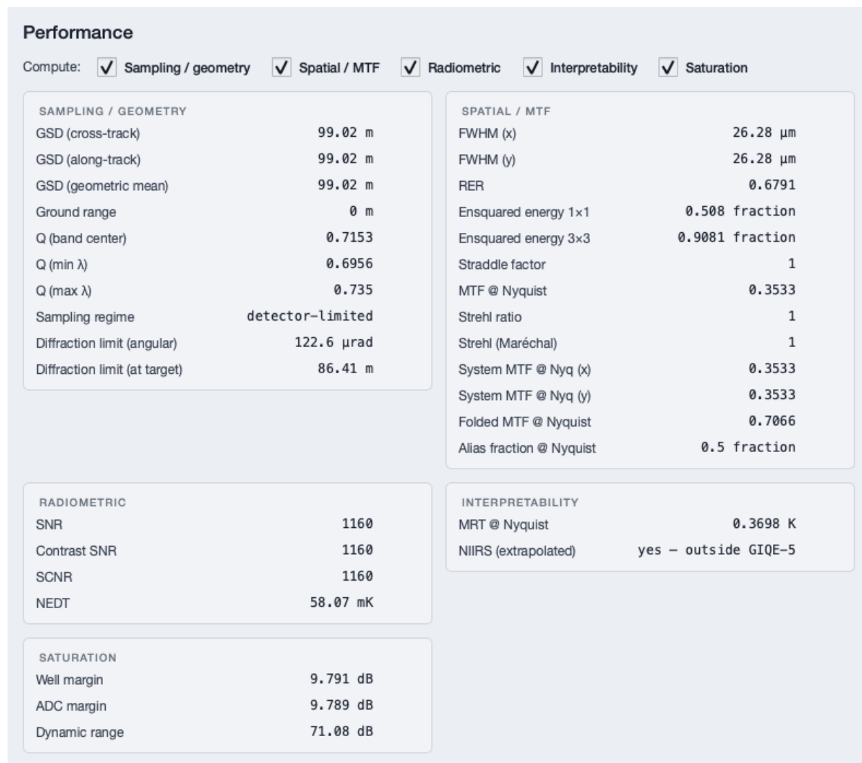
Figure 2.5: Performance workspace on the TIRS band-10 baseline. All five metric groups are enabled and populated.
