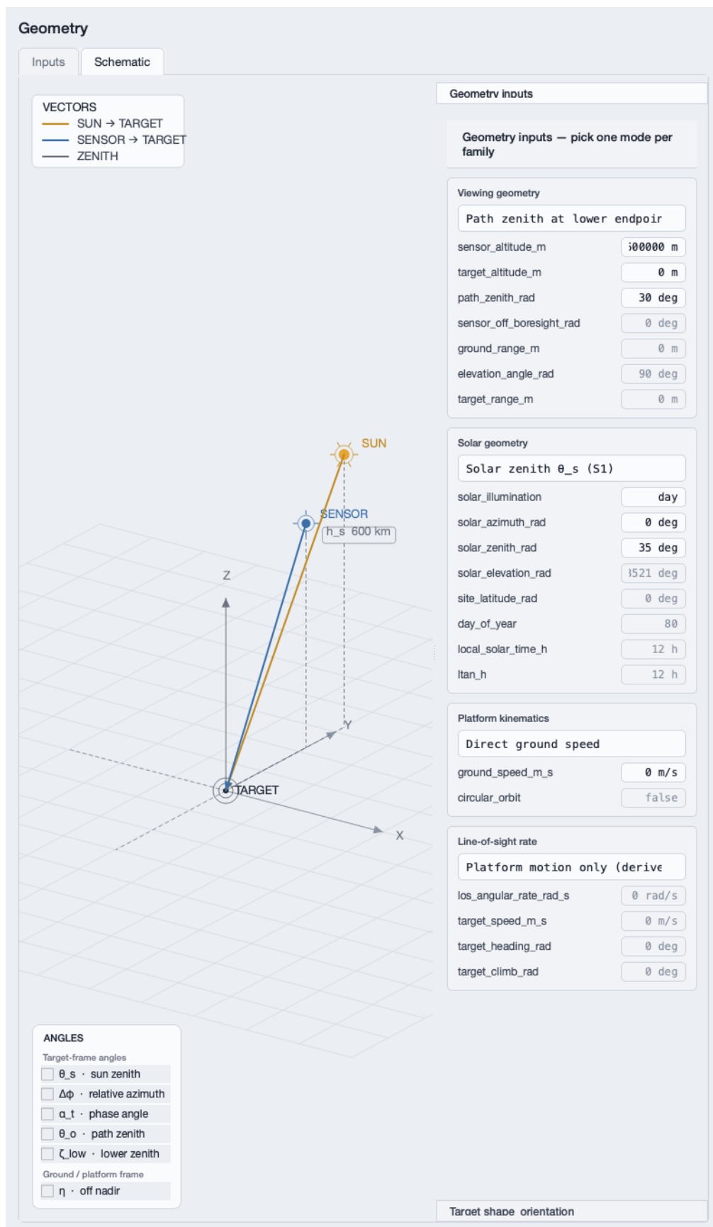
Figure 6.2: Geometry workspace, Schematic tab — the off-nadir look with the sun vector and the not-to-scale altitude leader pill.
