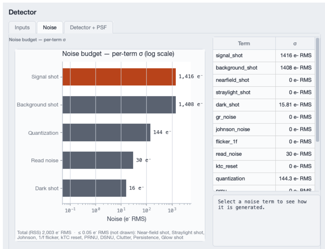
Figure 4.5: Detector workspace, Noise tab — the maritime noise budget, where background shot nearly matches signal shot.
