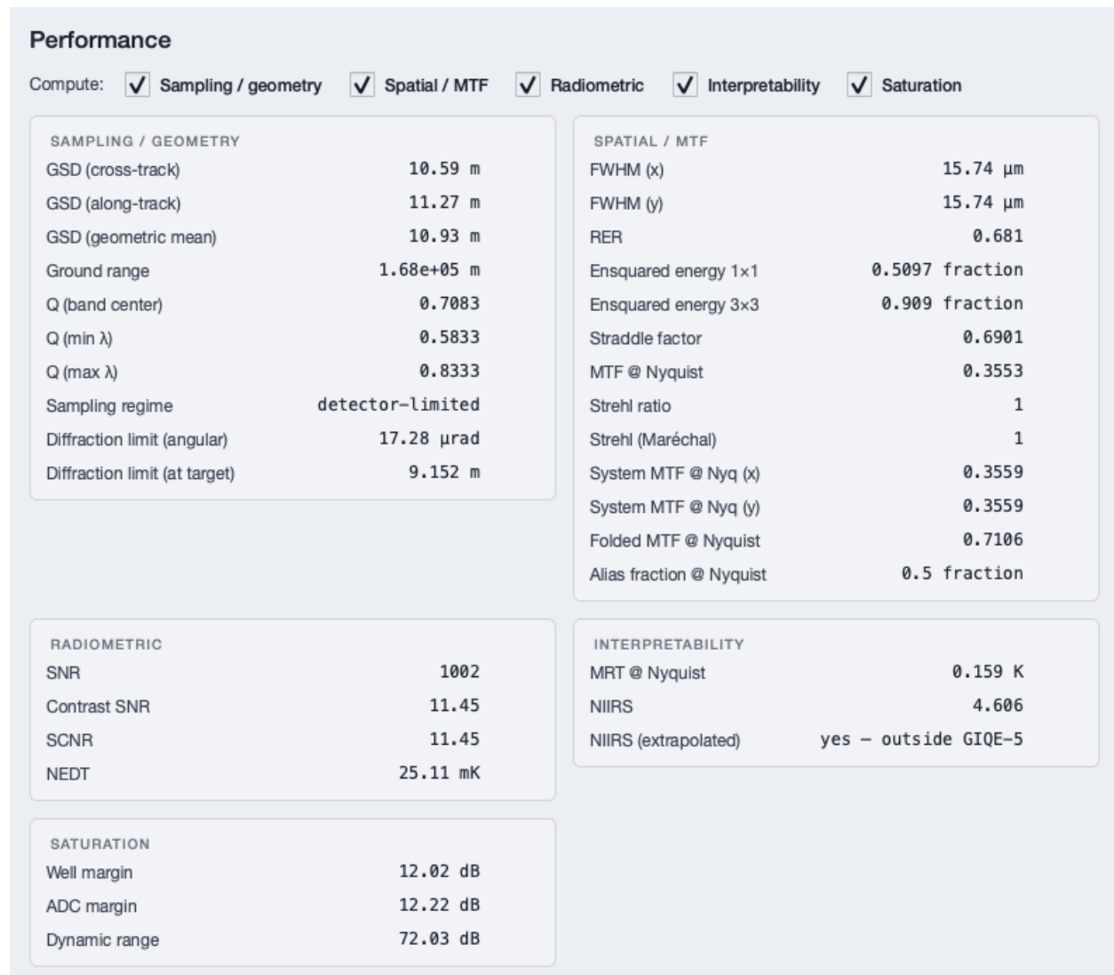
Figure 4.6: Performance workspace on the scenario 1.1 baseline — all five metric groups after evaluation.
