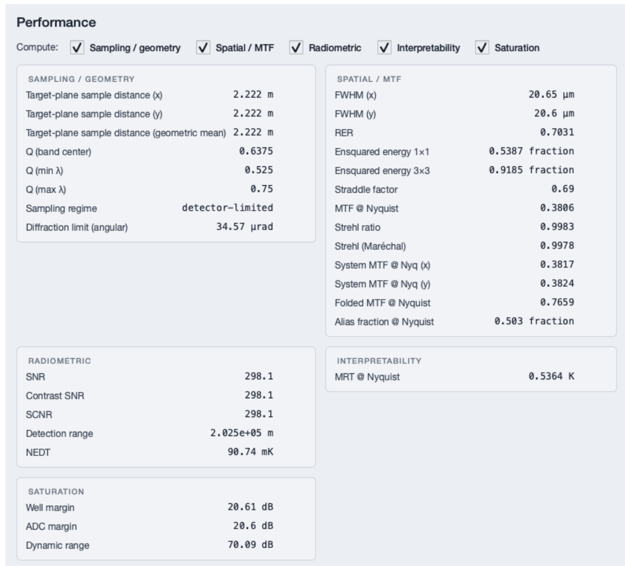
Figure 11.5: Performance workspace on the level arm — the ground-projection family absent by scene class, target-plane sample distance in its place.
