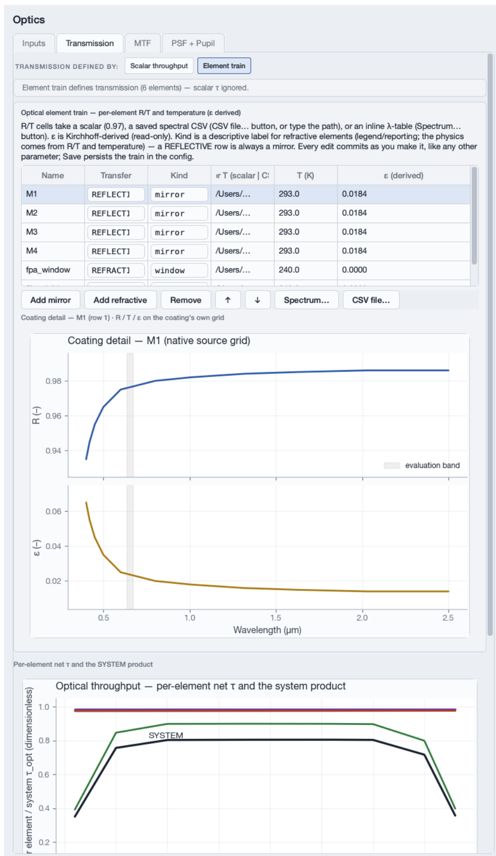
Figure 2.9: Optics workspace, Transmission tab — the element train as editable rows, with the selected element's coating curve beneath.
