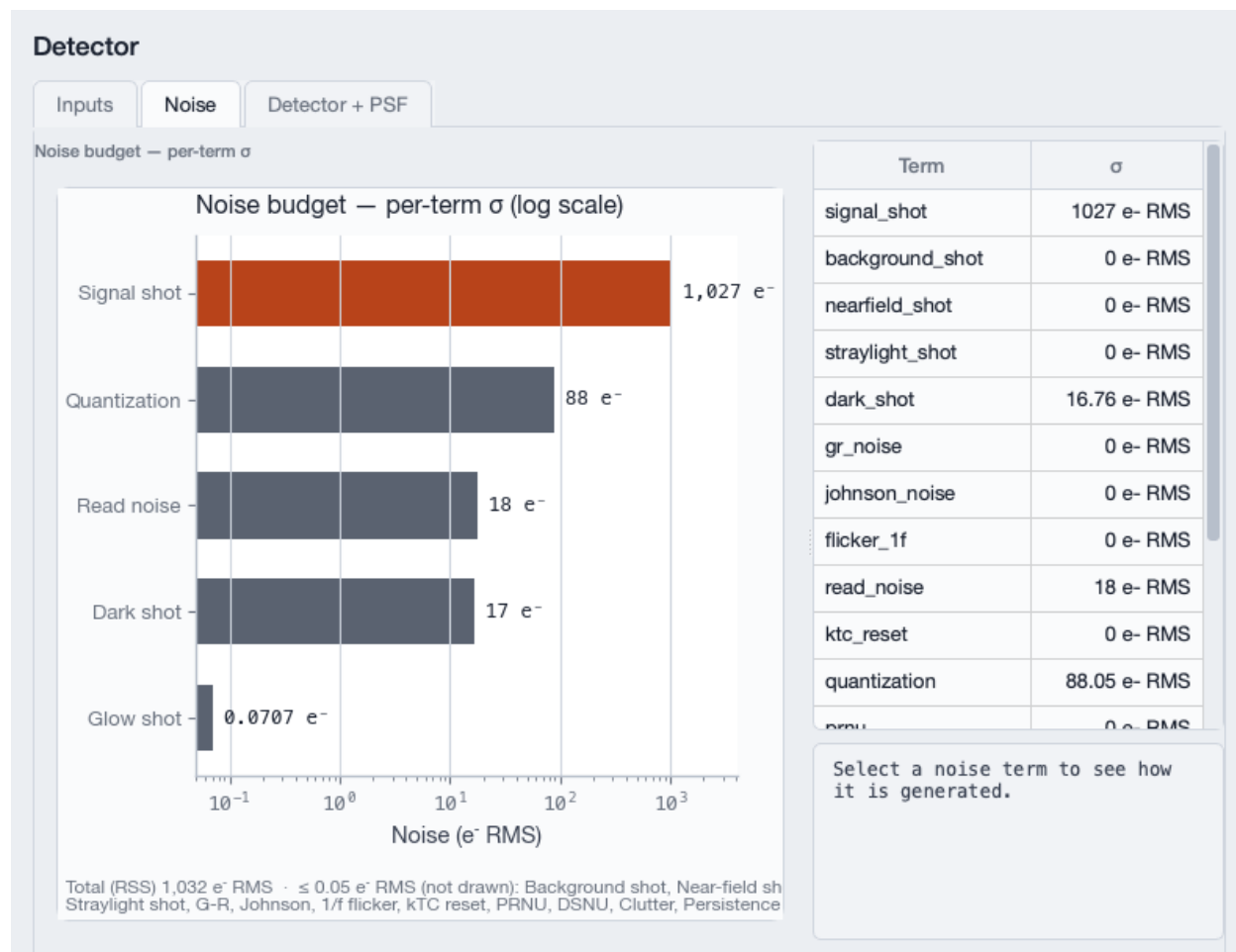
Figure 5.3: Detector workspace, Noise tab — the InSb bench budget, photon-limited, with quantization as the second term.
