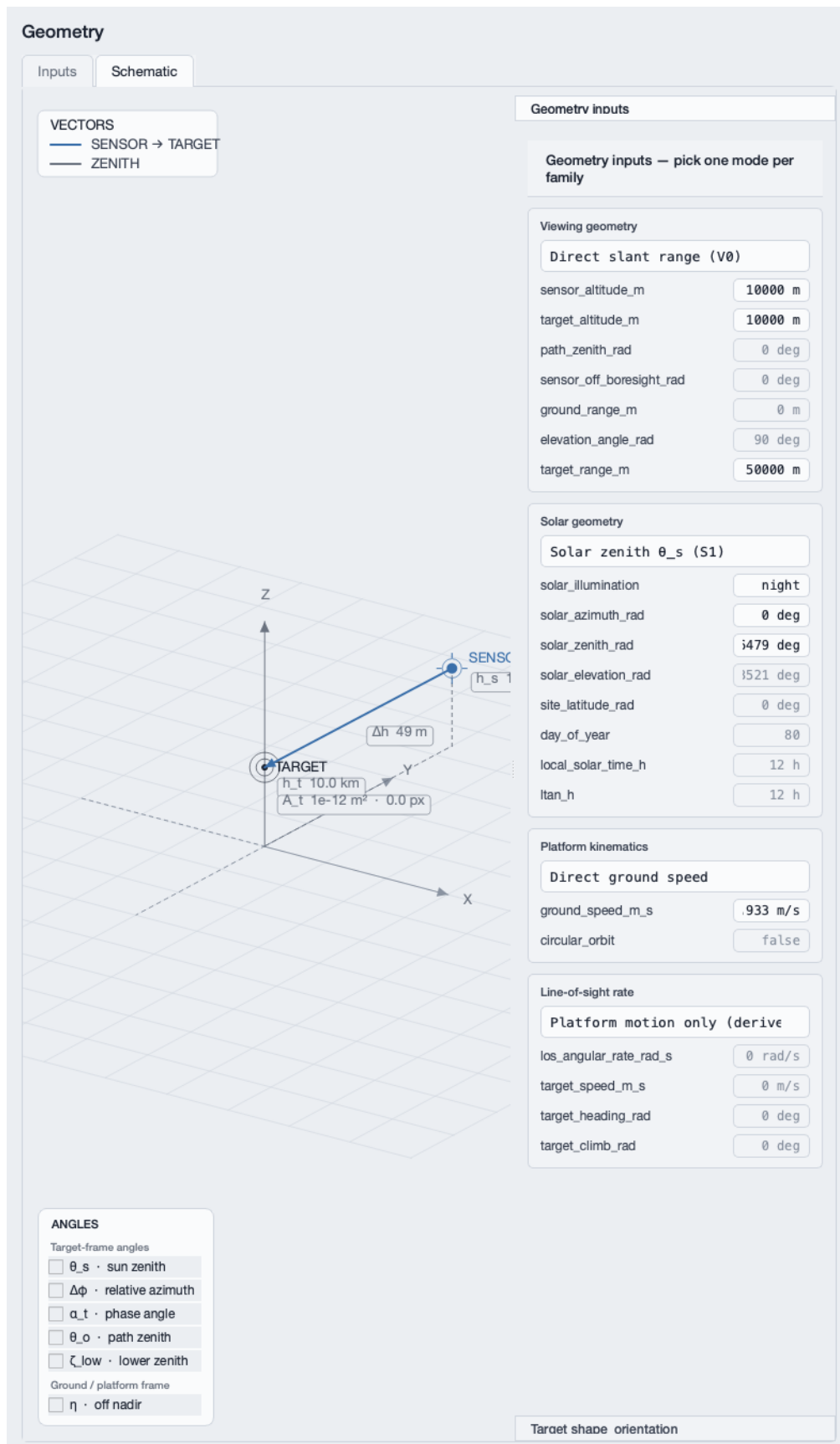
Figure 11.2: Geometry workspace, Schematic tab — the level composition, both endpoints at altitude, with the tangent-depression leader pill.
