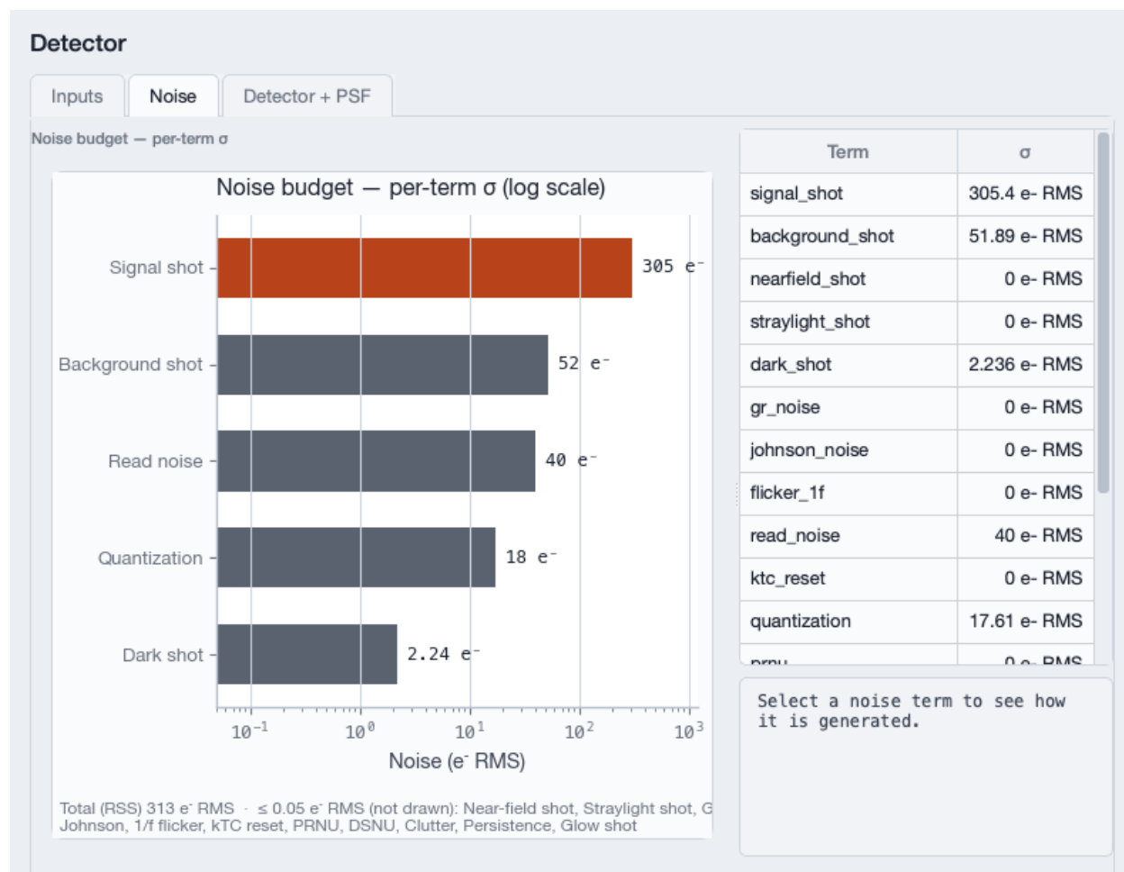
Figure 11.4: Detector workspace, Noise tab — the 50 km budget, dominated by the target's own shot noise.
