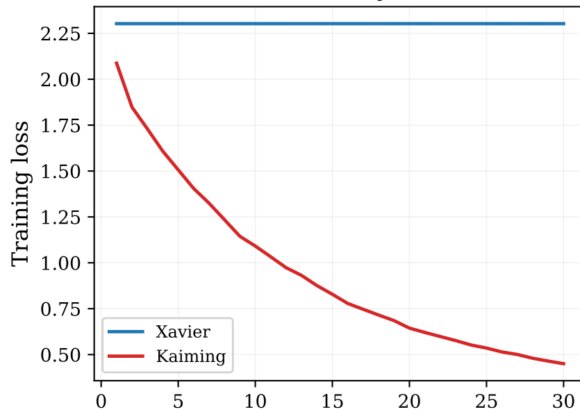
20 conv layers
