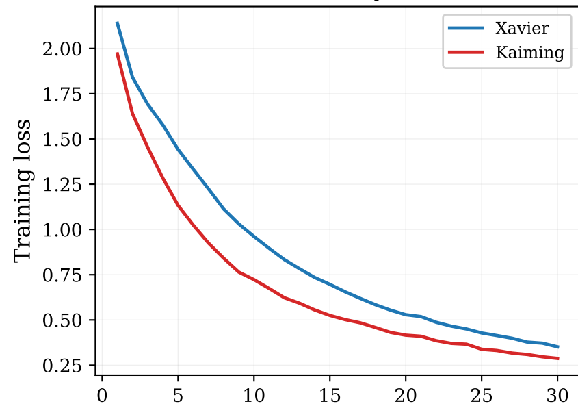
10 conv layers
