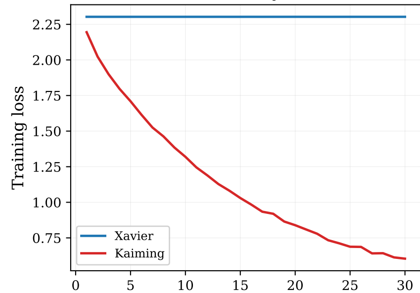
30 conv layers
