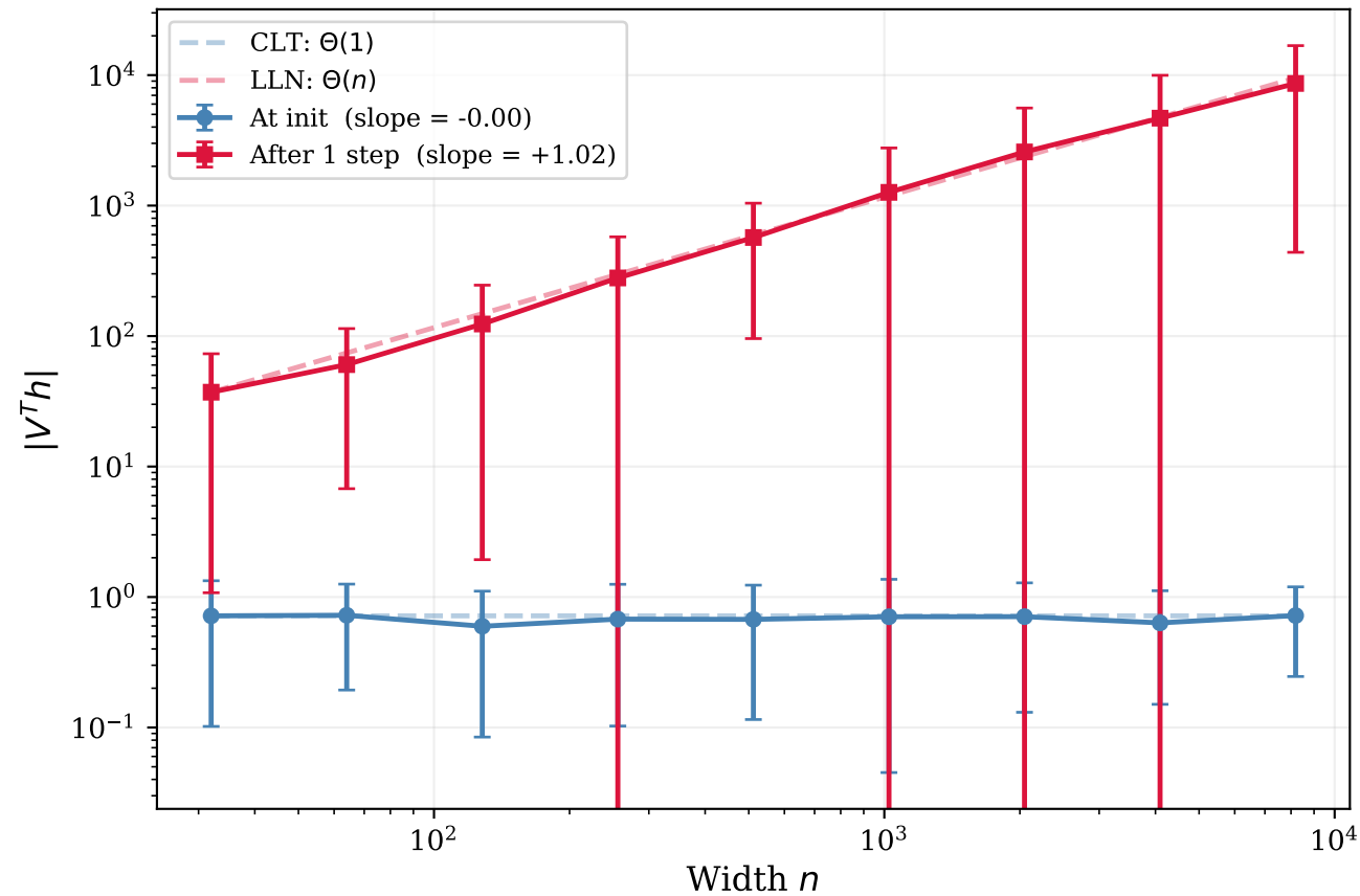
CLT (init, V \perp h ) vs LLN (after step, \mathcal{V} \perp h )
