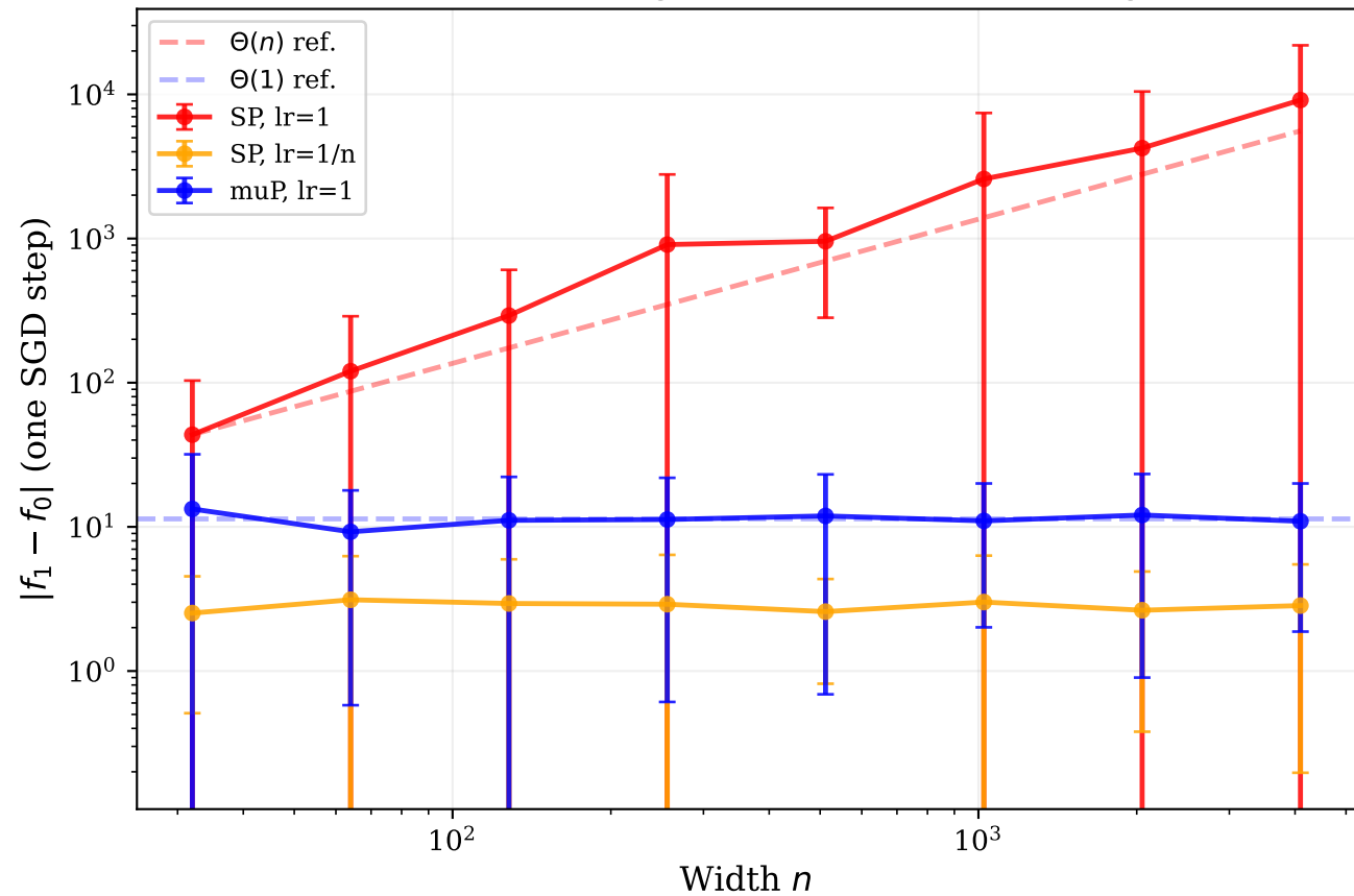
SP vs muP: scaling of one-step output change
