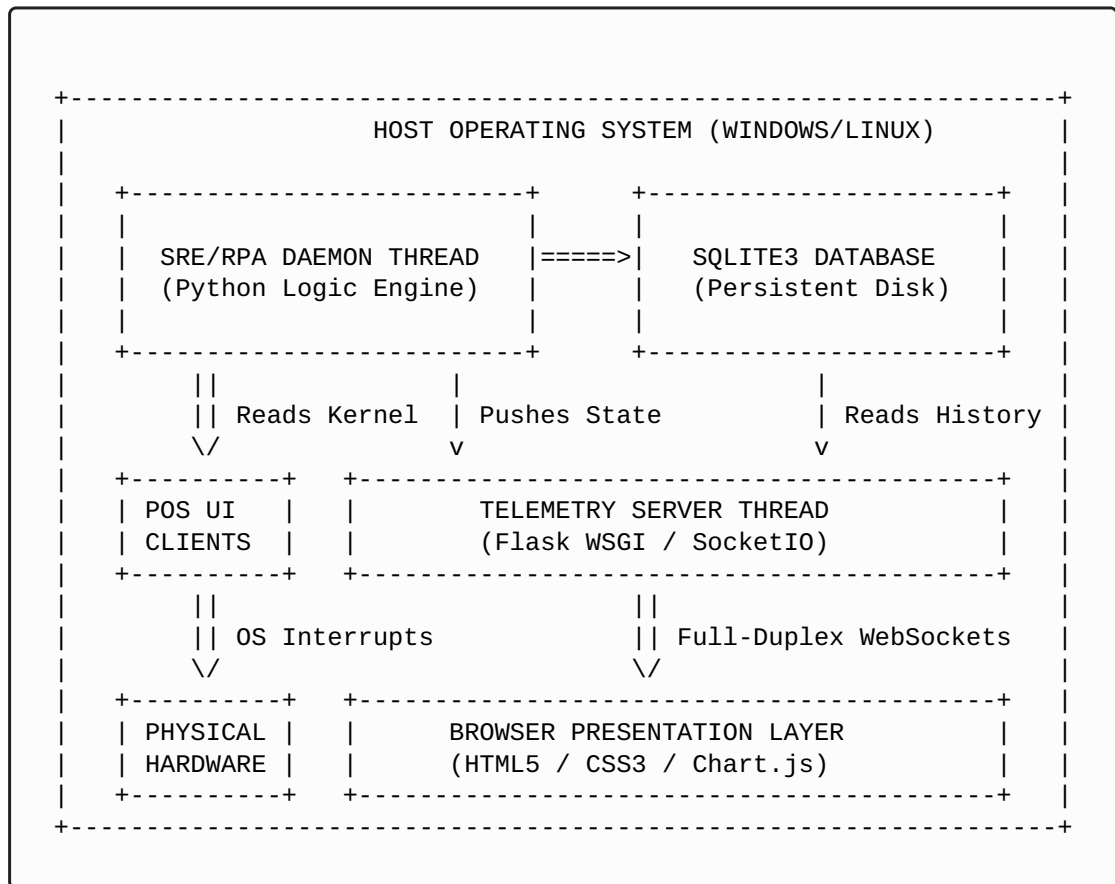
Figure 2.1: Macro System Architecture and Data Flow
