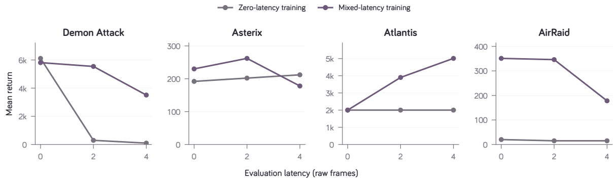
Figure 7 | Cross-task gains depend on the task and evaluation delay. Mixed-latency training on Demon Attack yields higher delayed returns on Atlantis and AirRaid, while Asterix has lower return at four frames than with zero-latency training. Gray and purple denote zero-latency and mixed-latency training, respectively. From left to right, panels show Demon Attack, Asterix, Atlantis, and AirRaid, evaluated at delays of 0, 2, and 4 raw frames. Each point is the mean episode return over 20 evaluation episodes.
