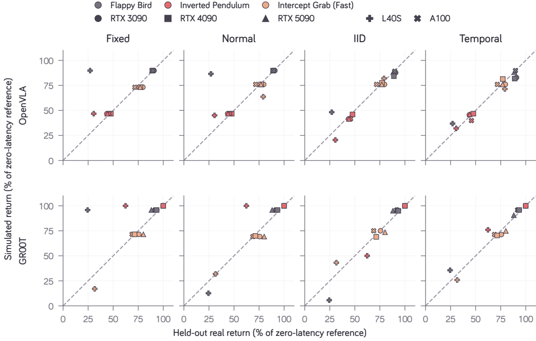
Figure 4 | Held-out sim-to-real calibration. We fit each latency profile on 25 hardware runs and test how well simulated returns predict 25 held-out hardware runs across 30 task–model–GPU cases. Rows show OpenVLA and GR00T; columns compare Fixed, Normal, IID, and Temporal profiles. Colors identify tasks, marker shapes identify GPU types, and the dashed line marks exact agreement. Temporal replay best matches hardware-timed performance, reducing normalized mean absolute error from 8.93 percentage points with Fixed replay to 3.81 percentage points.
