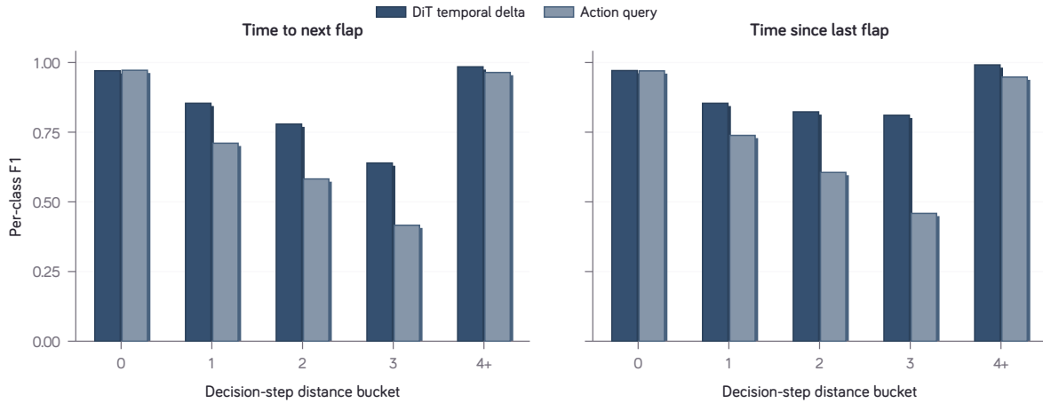
Figure 16 | After supervised fine-tuning, a linear classifier predicts action timing more accurately from diffusion-transformer (DiT) features than from action-query features. The left panel predicts decision steps to the next teacher flap; the right panel predicts steps since the previous flap. Bars are per-class F1 scores for distances 0, 1, 2, 3, and 4+, where 4+ combines all distances of at least four steps. DiT features have higher F1 in the 1-, 2-, and 3-step classes in both panels. Results use ordered five-frame input, one split with five training episodes and two validation episodes, and no confidence intervals. Class frequencies are imbalanced.
