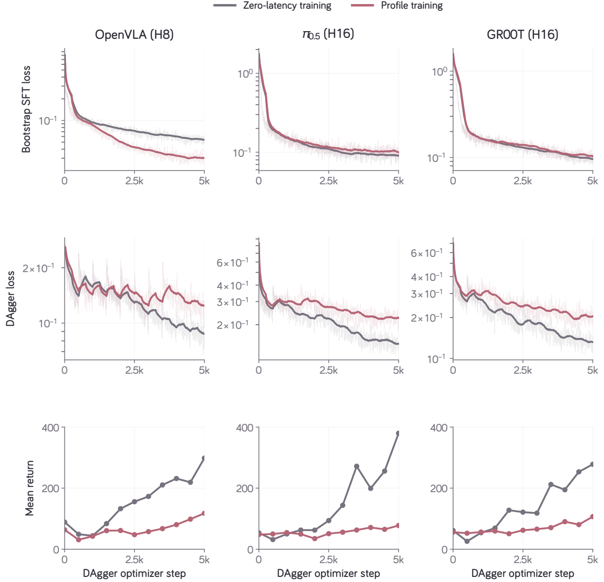
Figure 24 | Balance (simple) learning curves for action-chunk policies trained with DAgger. Columns show OpenVLA with eight predicted actions per call ( H = 8 ), and \pi_{0.5} and GR00T with sixteen ( H = 16 ). Gray and rose denote zero-latency training and training with the measured latency profile. The top rows show raw supervised and DAgger losses with 50-point trailing means on separate logarithmic axes; their absolute values are not comparable across architectures or training stages. The bottom row shows mean return on 32 fixed-seed development episodes, from the supervised endpoint at step 0 through 5,000 DAgger steps. All three architectures improve under both latency conditions, with larger increases in the zero-latency runs. Each curve is one training run.
