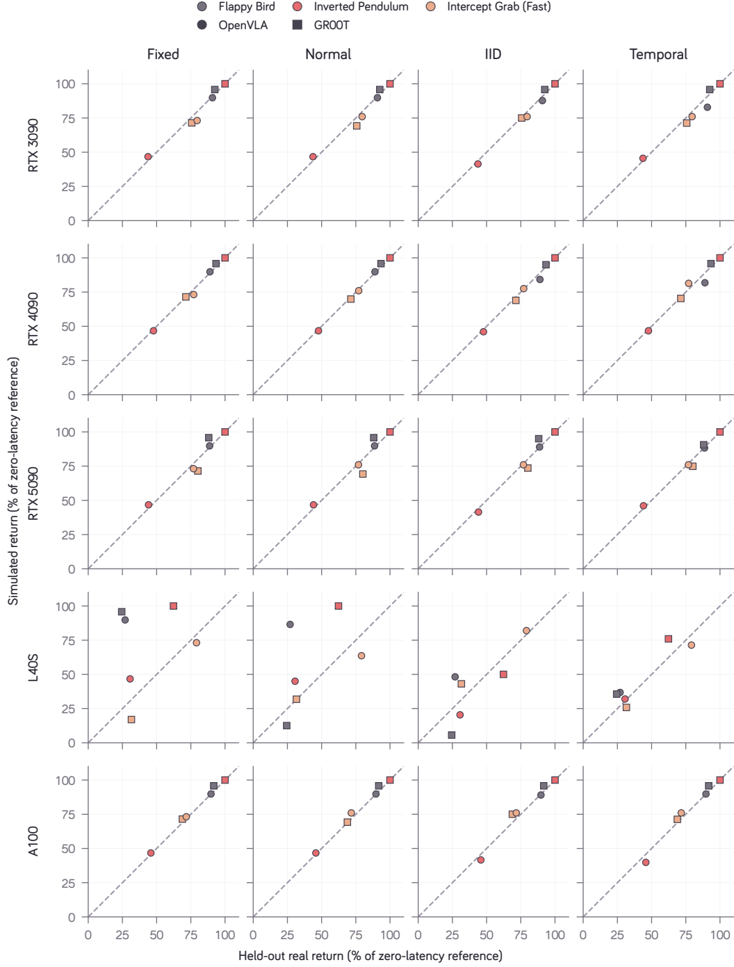
Figure 10 | Temporal replay closes most of the calibration gap on L40S. Its normalized mean absolute error (NMAE) falls from 34.75 percentage points for Fixed to 8.25 for Temporal, averaged equally across six cases. Rows identify GPU types; columns compare Fixed, Normal, IID, and Temporal. Colors identify Flappy Bird, Inverted Pendulum, and MIKASA Intercept Grab (Fast); marker shapes identify OpenVLA and GR00T. Each point is one task–model case. Both axes report mean return as a percentage of the same task/model zero-latency-trained policy reference. Profiles use 25 fitting runs; points average 25 held-out runs with two consecutive episodes per run. The dashed line marks exact agreement.
