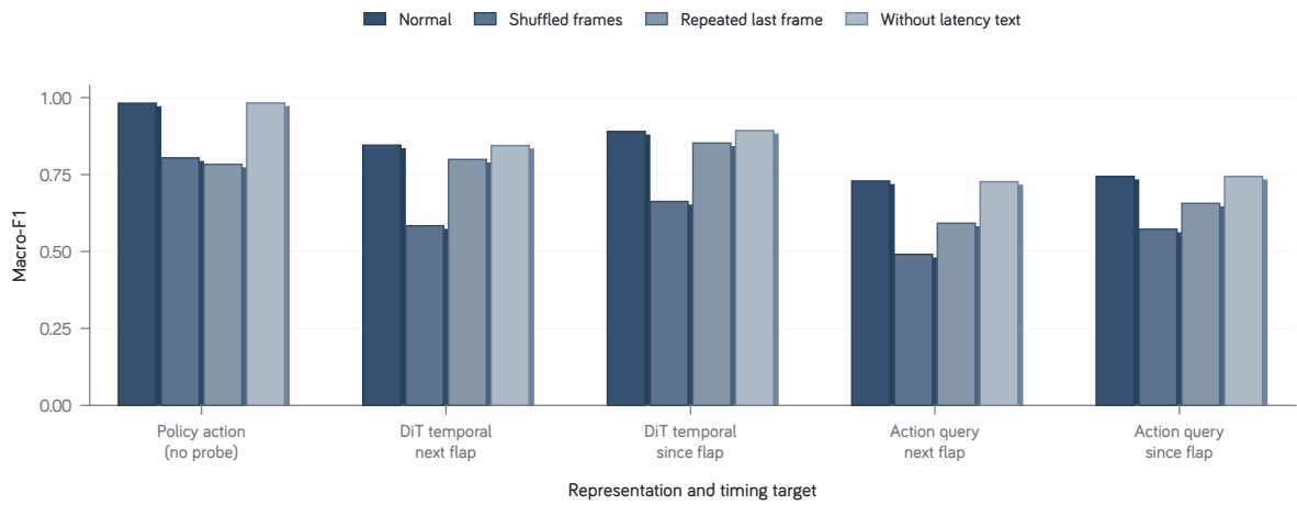
Figure 15 | A linear classifier predicts flap timing more accurately from WanOFT features when the five input frames remain in temporal order. Bars report validation Macro-F1, the mean F1 score across timing classes, for predicting the number of decision steps to the next teacher flap or since the previous flap. Policy action is the model’s direct output; all other bars use a separate linear classifier trained on frozen features for the displayed input condition. DiT refers to features from the diffusion-transformer backbone. Shuffling frame order reduces post-SFT next-flap Macro-F1 from 0.845 to 0.584 for DiT features and from 0.729 to 0.491 for action-query features. The experiment measures what timing information a classifier can read from the representation, not whether the policy uses that information to act. Results use a single fixed delay of 2 frames, five training episodes, and two validation episodes, so they do not test generalization across latency values.
