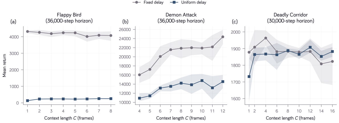
Figure 13 | Increasing visual-history length does not improve all tasks under latency. The horizontal axis is context length C , implemented by stacking the latest C observation frames. Fixed delay is 2 frames for Flappy Bird and 4 frames for the other tasks. Uniform delay samples 1–3 frames for Flappy Bird and 2–6 frames for the other tasks. Each point averages the mean returns of five independently trained policies; shading is a 95% bootstrap confidence interval obtained by resampling those five training seeds. Each policy is trained and evaluated with the same profile.
