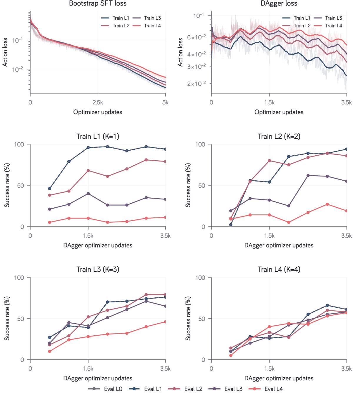
Figure 23 | OpenVLA H8 learning curves for MIKASA policies trained at fixed delays of 1, 2, 3, or 4 frames. The top panels show 50-record trailing means of the supervised and DAgger losses on logarithmic axes. The bottom panels correspond to the four training delays; within each panel, line color denotes the evaluation delay. Each success-rate point averages the same 100 development episodes, beginning at update 500. The action prefix contains actions already queued for execution. Its length K equals the policy’s training delay and remains fixed when the evaluation delay changes. Supervised training runs for 5,000 updates and DAgger for 3,500; each trajectory is one training run.
