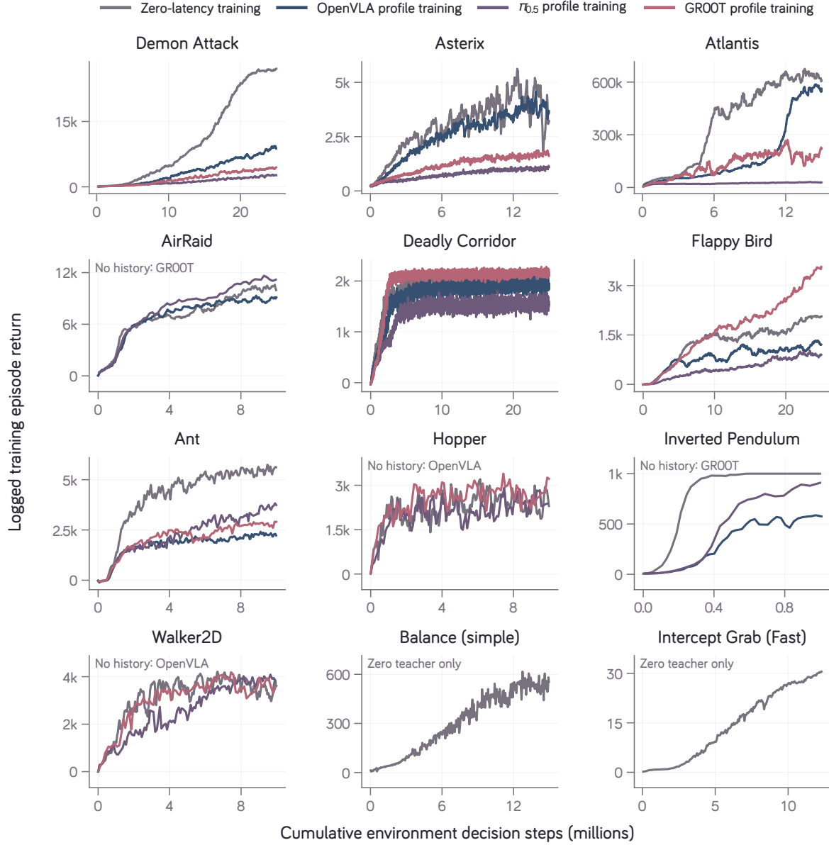
Figure 18 | Learning curves for the task-specific RL teachers used to label VLA training data. The horizontal axis is the number of environment steps and the vertical axis is mean episode return. Each curve is one training run under either zero latency or the displayed deployment profile. Environment rates and episode limits differ across conditions, so differences in curve height should not be interpreted as the isolated effect of latency.
