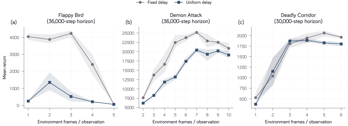
Figure 12 | The observation stride that gives the highest return depends on the task and latency profile. The horizontal axis is the number of environment frames between policy observations and action updates, so a smaller stride means more frequent control. Fixed delay is 2 frames for Flappy Bird and 4 frames for the other tasks. Uniform delay samples 1–3 frames for Flappy Bird and 2–6 frames for the other tasks. Each point averages the mean returns of five independently trained policies; shading is a 95% bootstrap confidence interval obtained by resampling those five training seeds. Each policy is trained and evaluated with the same profile.
