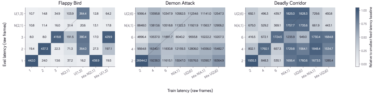
Figure 11 | No training profile gives the highest return across all tasks and evaluation profiles in this small-policy sweep. Columns specify the training profile and rows specify the evaluation profile; the dashed diagonal marks cells that use the same single profile for training and evaluation. N(\mu, \sigma) is a clipped Normal distribution over frame delays, and U(a, b) samples integer delays uniformly from a to b ; Mix denotes training across multiple listed conditions. Cell labels are mean returns over three training seeds. Within each task, color divides the cell value by the result obtained when the smallest fixed delay is used for both training and evaluation: (1, 1) for Flappy Bird and (2, 2) for the other tasks. Episode limits are 3,600 steps for Flappy Bird, 36,000 for Demon Attack, and 30,000 for Deadly Corridor.
