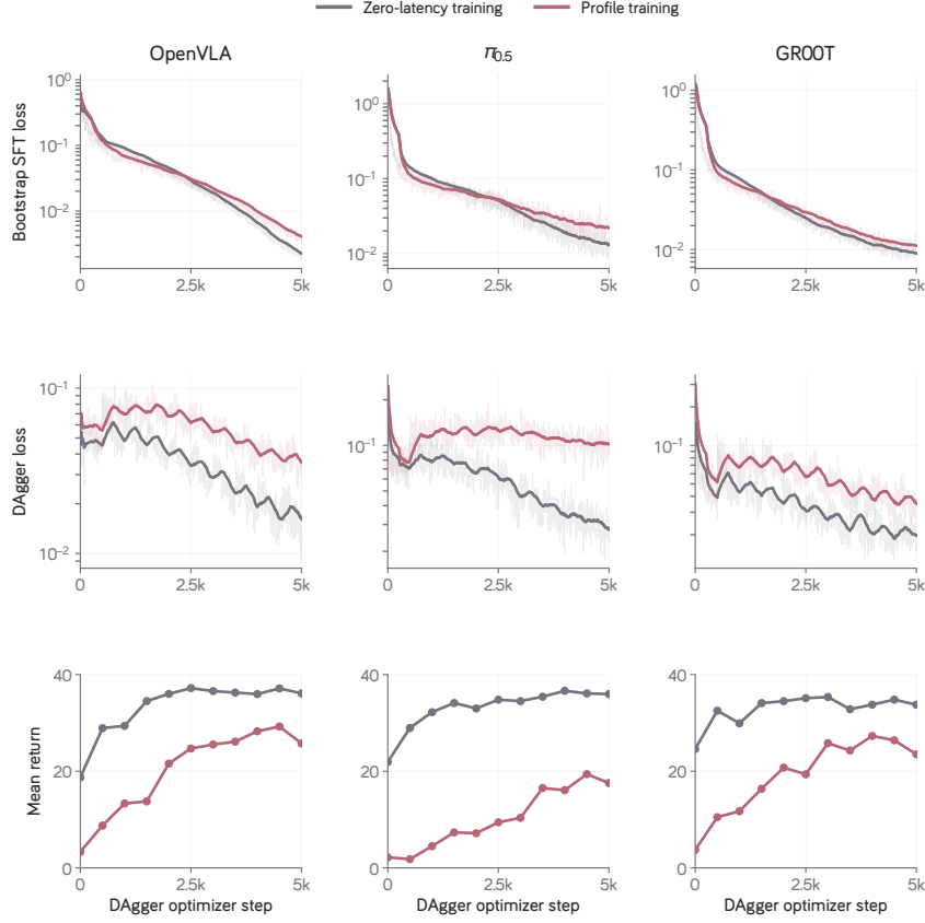
Figure 21 | MIKASA eight-action DAGger learning curves under Zero-latency training and Profile training. Columns correspond to the three VLA architectures. The top and middle rows show the training losses displayed in each panel; the bottom row shows mean return during training. Each return point averages the same 100 development episodes, except steps 0 and 5,000, which use a separate set of 200 episodes. Each curve is one training run. The endpoint is the final checkpoint, while Figure 1 reports the best checkpoint.
