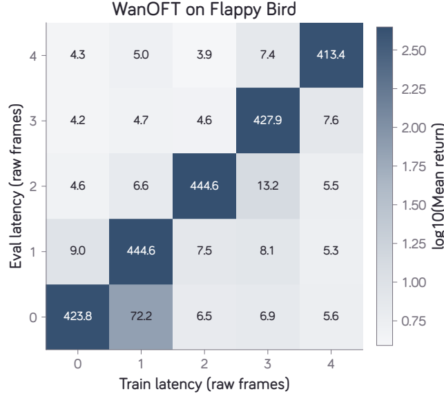
Figure 14 | WanOFT performs well mainly when its training and evaluation delays match, despite receiving five observation frames. Columns are fixed training delays and rows are fixed evaluation delays, both from 0 to 4 raw frames on Flappy Bird. Cell labels give mean episode return over 20 evaluations, and color shows \log_{10}(\max(\bar{R}, 1)) . Each policy receives the current frame and the preceding four frames, uses one training seed, and is evaluated for at most 3,600 steps per episode. At 30 FPS, one raw frame is 33.33 ms. Uncertainty is not shown.
