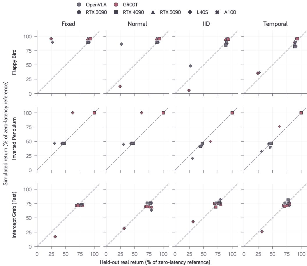
Figure 9 | Temporal profiles give the lowest replay error on Flappy Bird and Inverted Pendulum. Rows show Flappy Bird, Inverted Pendulum, and MIKASA Intercept Grab (Fast); columns compare Fixed, Normal, IID, and Temporal. Colors identify OpenVLA and GR00T; marker shapes identify GPU types. Each point is one model–deployment case. Both axes report mean return as a percentage of the same task/model zero-latency-trained policy reference. Profiles use 25 fitting runs; points average 25 held-out runs with two consecutive episodes per run. The dashed line marks exact agreement. Normalized mean absolute error (NMAE) gives each case equal weight.
