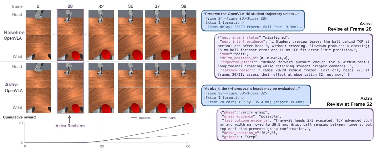
Figure 17 | One selected MIKASA episode shows GPT-6 Astra choosing a correction after the unreviewed OpenVLA action misses the object. The left side compares head and wrist views from the baseline rollout with the reviewed rollout; the plotted value is reward accumulated up to each frame. OpenVLA predicts an action chunk, a geometry module proposes a slower correction, and Astra (OpenAI, 2026) selects whether to apply it given a stated 100 ms delay. The abridged interaction on the right shows the correction at frame 28 and review of the possible grasp at frame 32. This is a qualitative example, not an estimate of average success rate. Simulation pauses during the Astra API call, so the example does not test real-time intervention.
