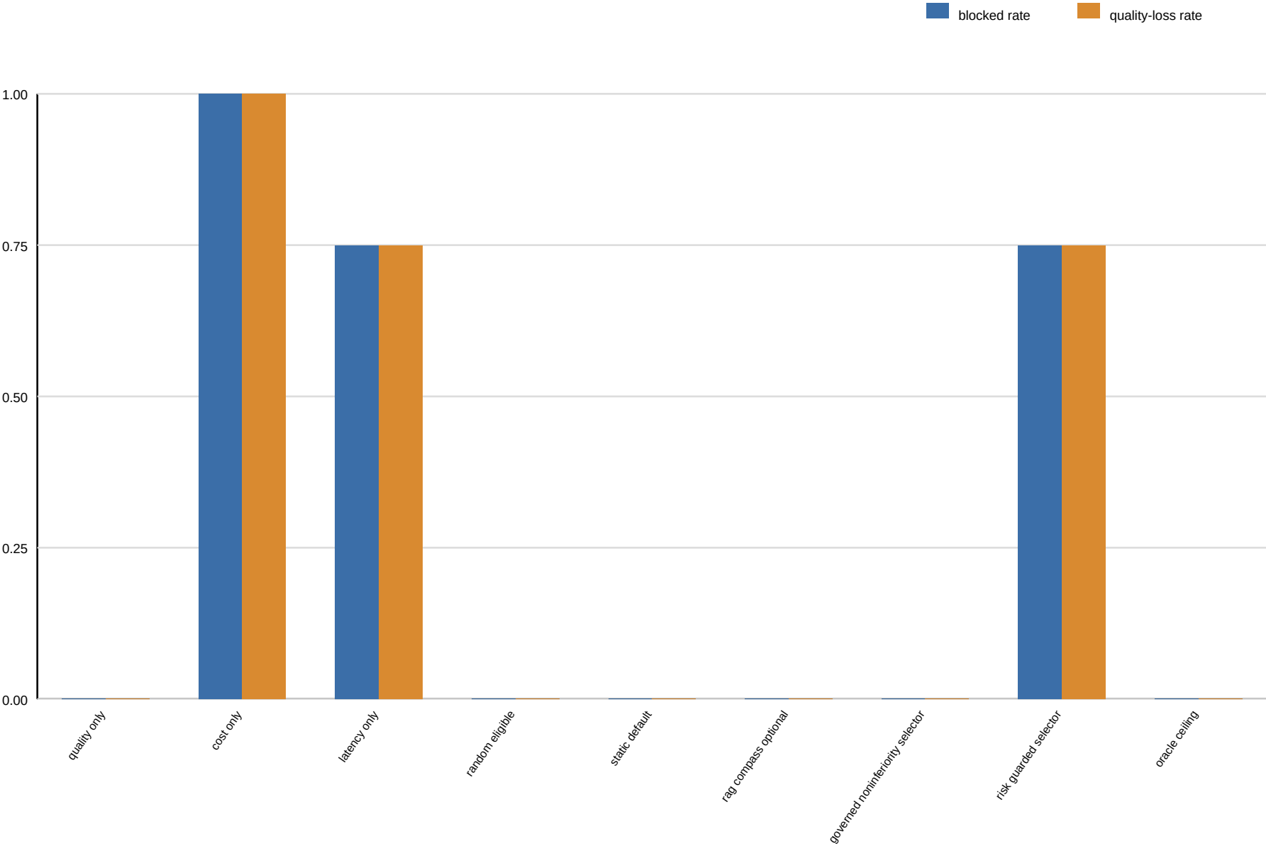
Selector stress test: blocked rate and quality-loss rate
