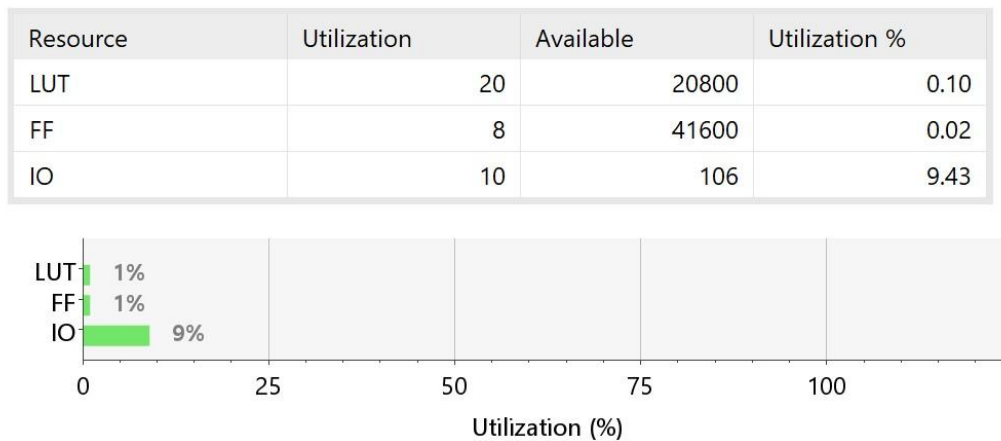
Figure 3.5: Resource Utilization Report
