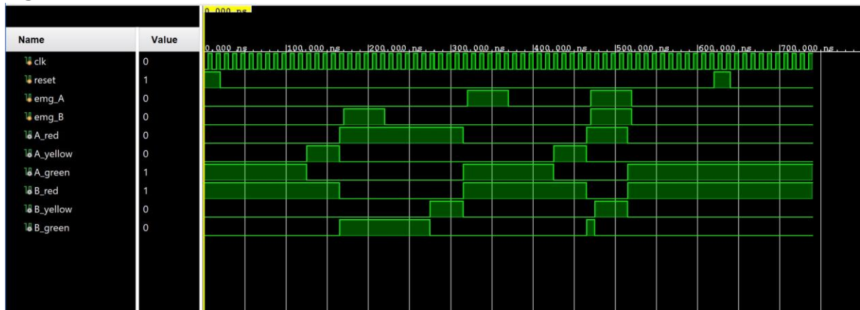
Figure 3.2: Behavioral Simulation Waveform
