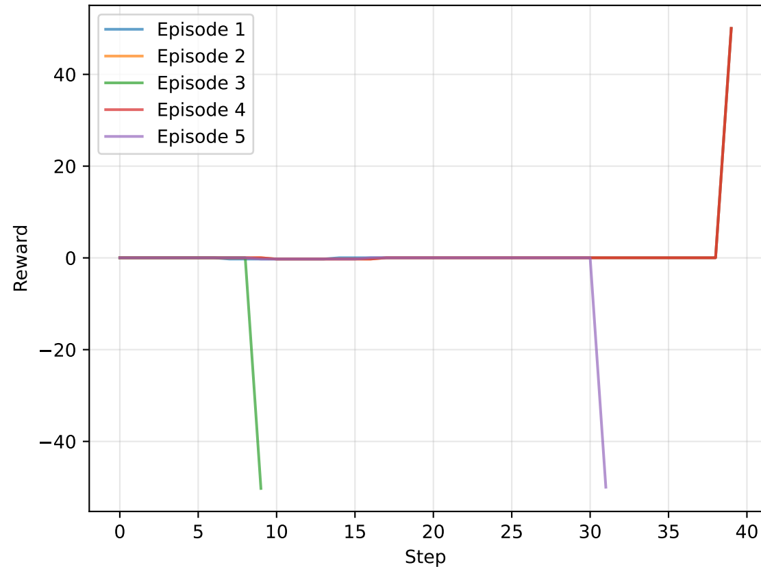
Reward Trajectories (First 5 Episodes)
