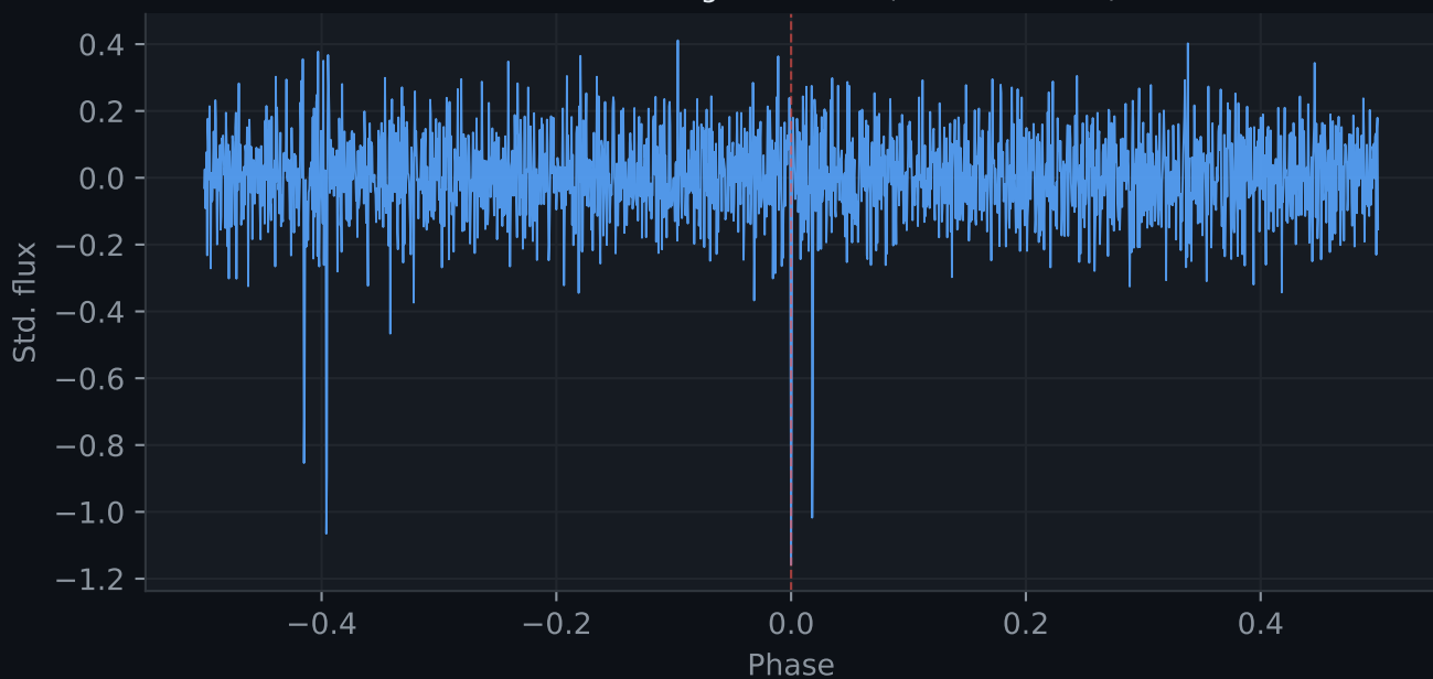
KIC 6431670 — global view (P = 14.9539 d)
