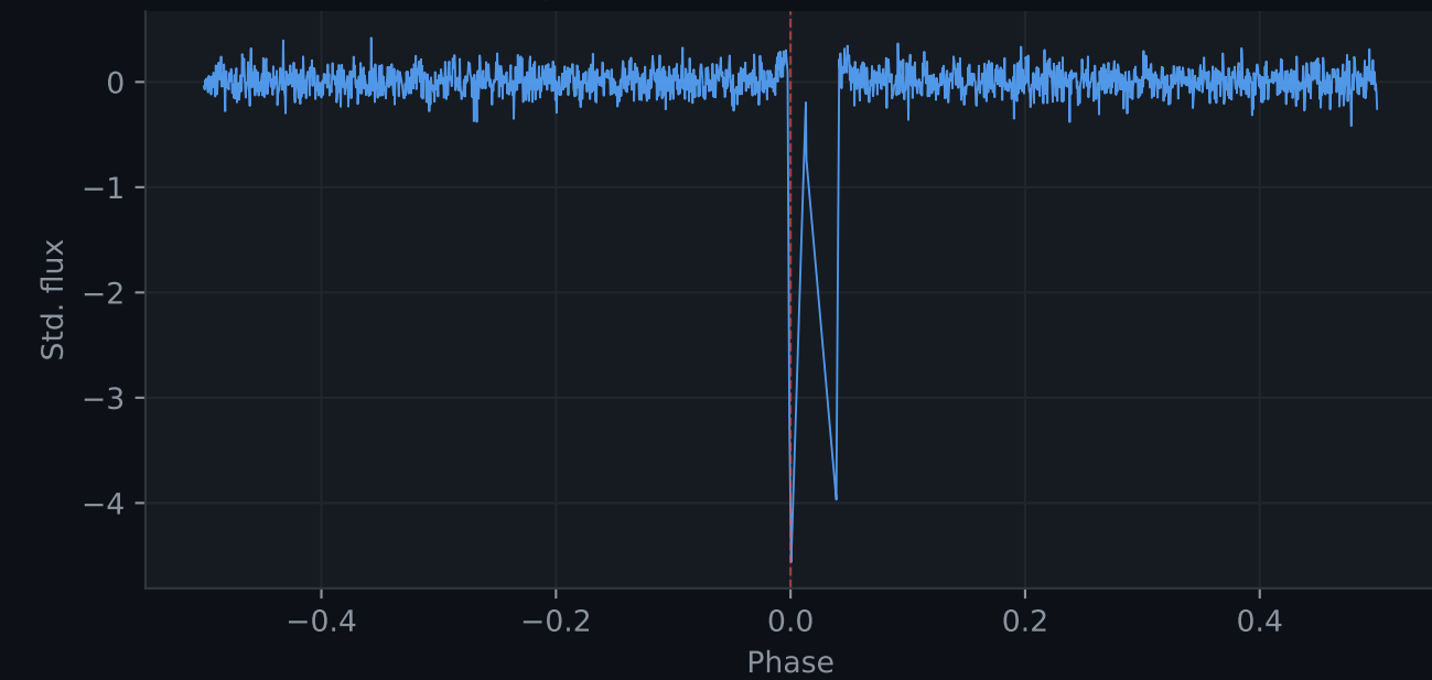
Kepler-20 — global view (P = 10.8530 d)
