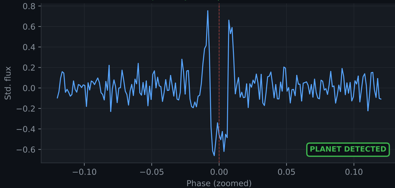
Super-Earth [cascade] | Confidence: 91.20%
