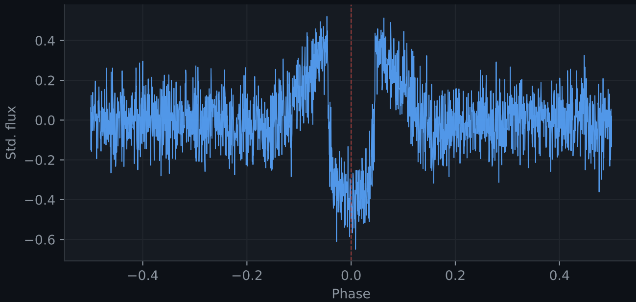
Kepler-7 — global view (P = 4.8855 d)
