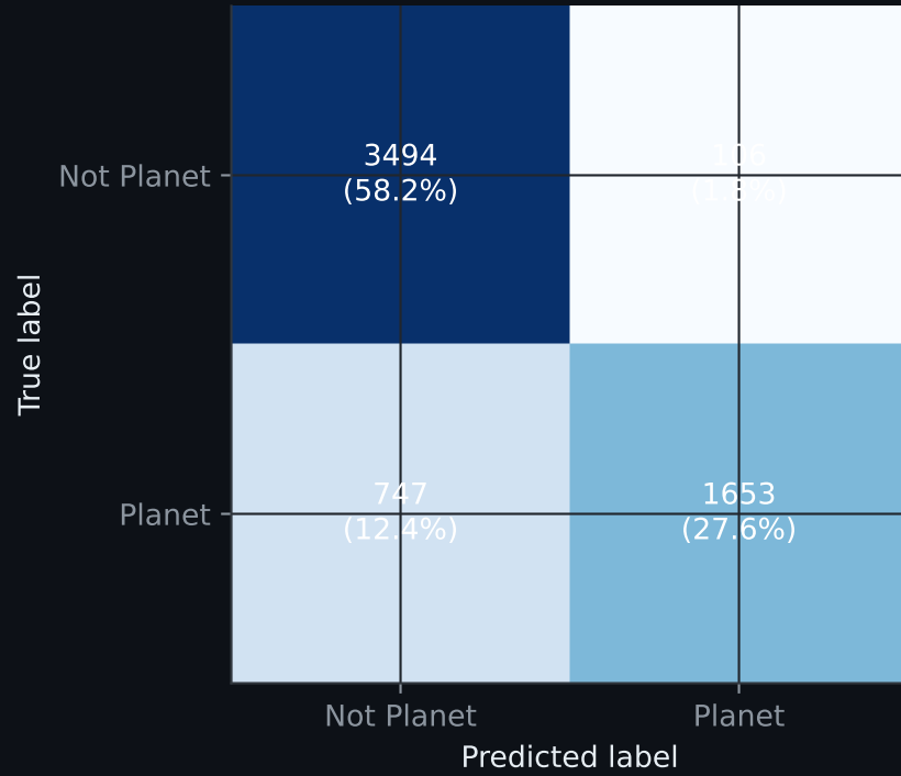
Confusion Matrix
