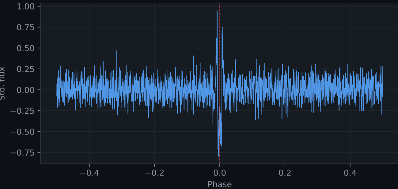
Kepler-62 — global view (P = 5.7153 d)
