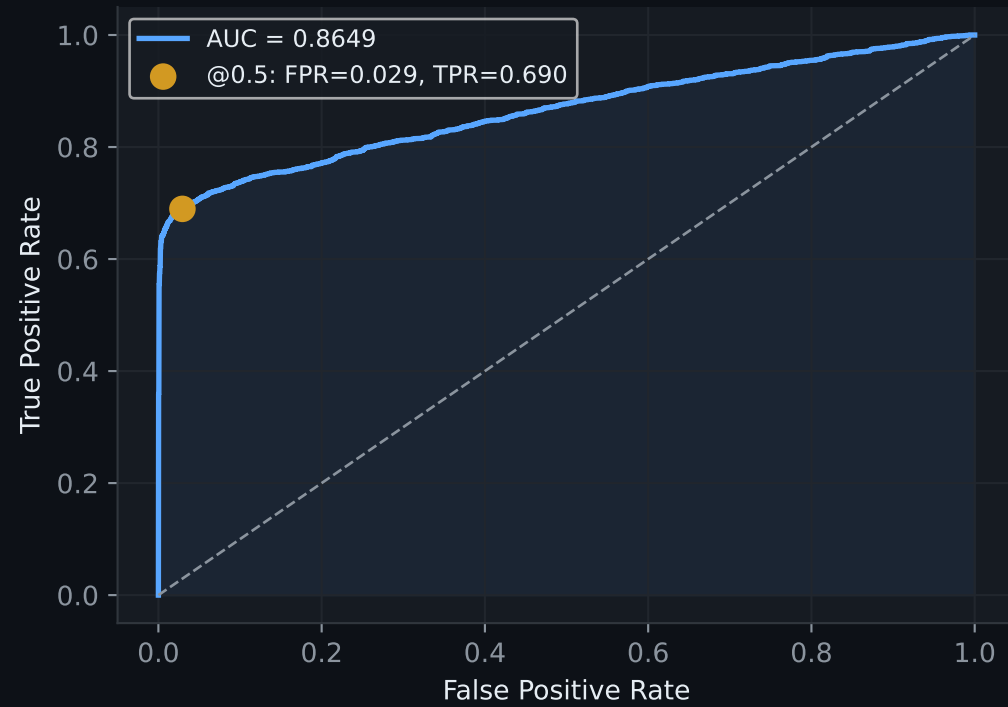
ROC Curve
