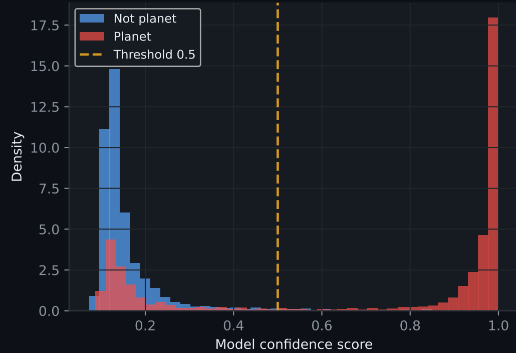
Confidence Score Distribution
