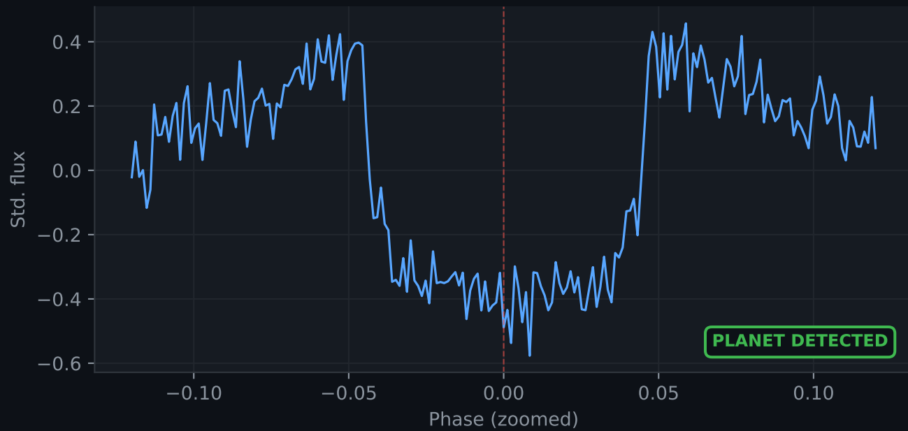
Hot Jupiter — 4.89 d | Confidence: 94.88%
