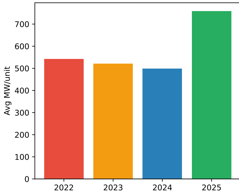
showers
