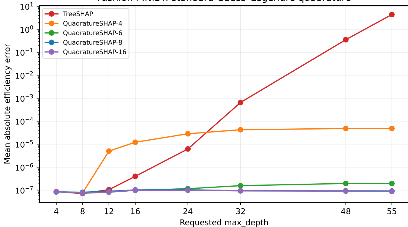
Fashion-MNIST: standard Gauss-Legendre quadrature
