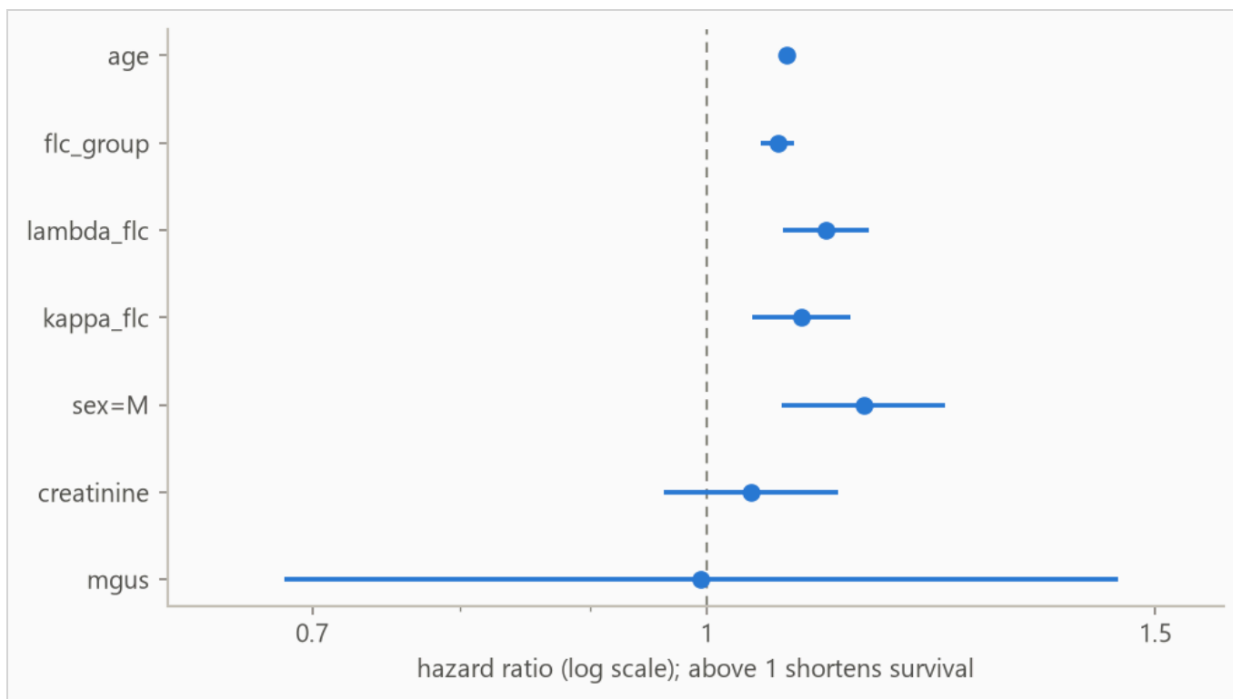
Figure 7. Hazard ratios for the strongest Cox covariates on a log axis, so a doubling and a halving of risk sit the same distance from the dashed no-effect line at 1.0.
