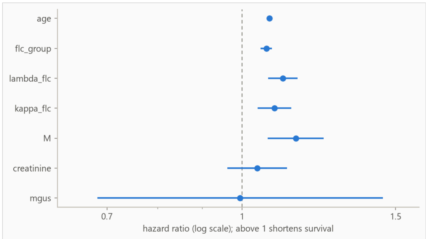
Figure 6. The Cox Proportional Hazards model's strongest covariates with their 95% intervals on a log axis. Dots right of the line shorten survival and left lengthen it. The covariate whose effect the data pins down most firmly sits at the top, and only the strongest few are drawn. Ratios for sex compare against F (automatically chosen alphabetically) and excluded from the fit.
