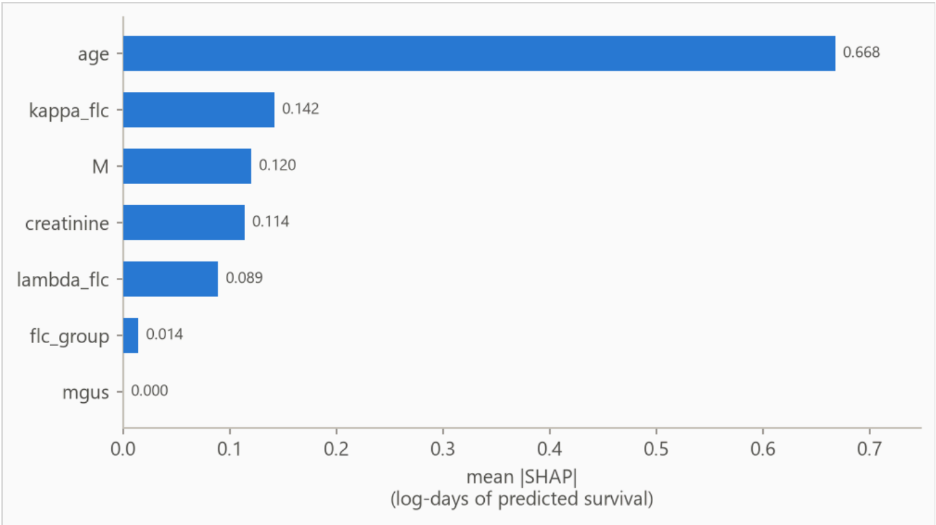
Figure 4. The strongest features, ranked by the average size of their attributions across the explanation sample. Size is taken without regard to sign, so this says how much each feature moves predictions and not which way it moves them; the direction is in Figure 5. The scale is the same log scale of survival time, so a feature averaging 0.10 moves predicted survival time by about a tenth on a typical row. A yes/no flag from a text column is labelled by its value alone. Features below the strongest few are not drawn.
