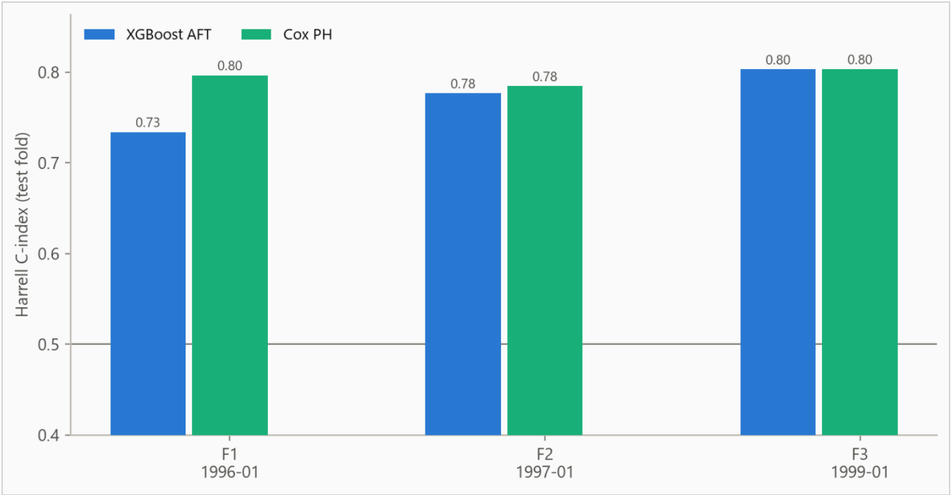
Figure 2. Concordance by fold. The boosted model spans 0.734 to 0.803. Folds differ in censoring mix, so cross-fold comparisons are indicative rather than exact.
