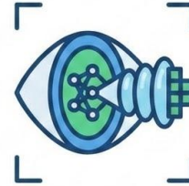
Computer Vision
