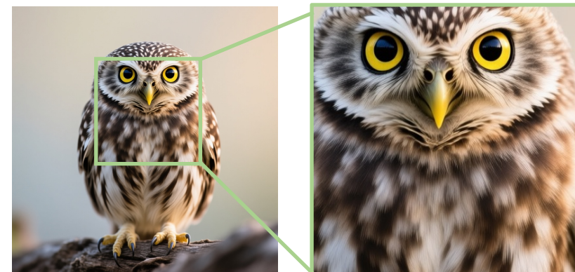
GradHarmon
