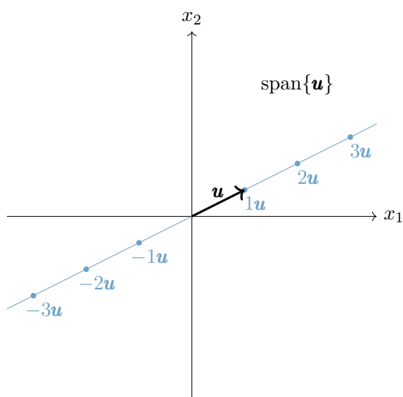
(a) The span of one vector in \mathbb{R}^2 is a line through the origin.
