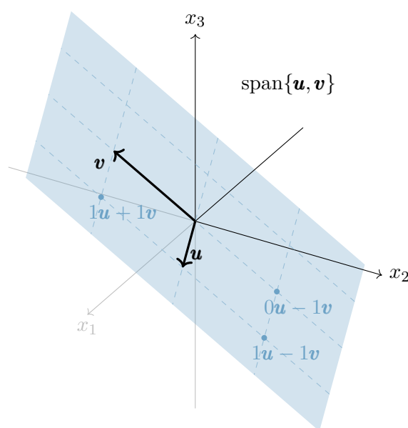
(b) The span of two non-parallel vectors in \mathbb{R}^3 is a plane through the origin.
