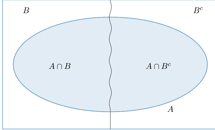
Figure 5.1: P(A) = P(A \cap B) + P(A \cap B^c)
