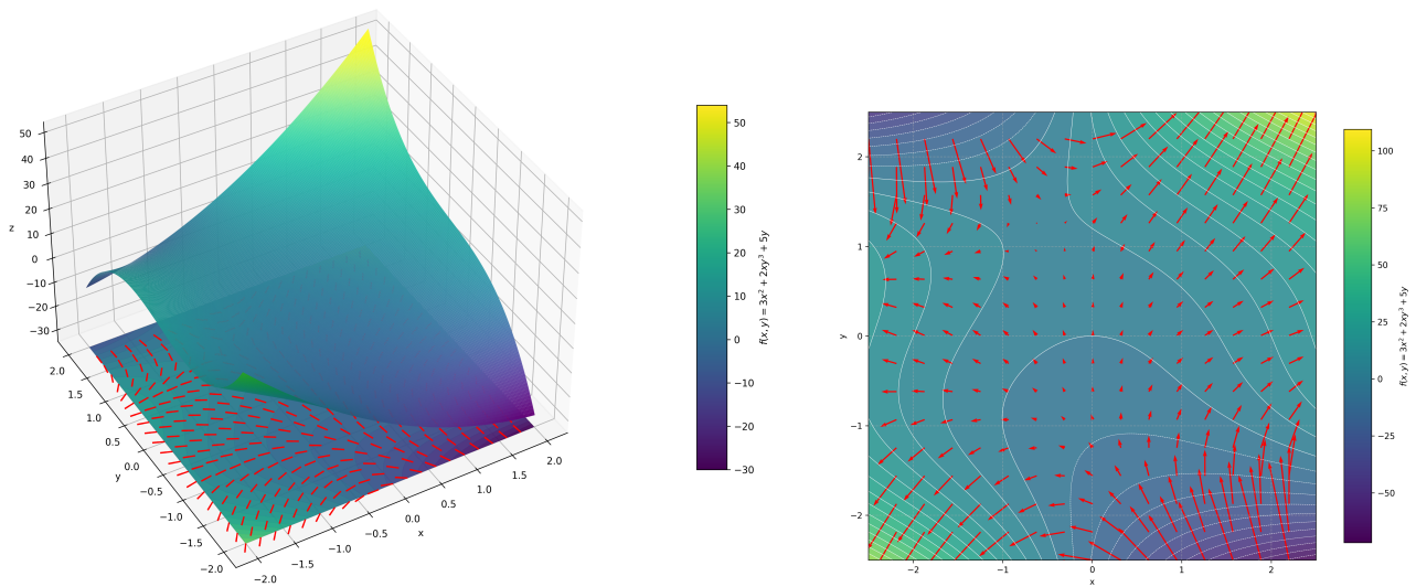
(a) A 3D view of the surface z = f(x, y) with its gradient field projected below.
