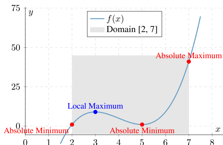
Figure 10.9: On the restricted domain [2, 7] , the absolute maximum occurs at an endpoint ( x = 7 ), not at the local maximum. The absolute minimum occurs at both the endpoint x = 2 and the interior stationary point x = 5 .
