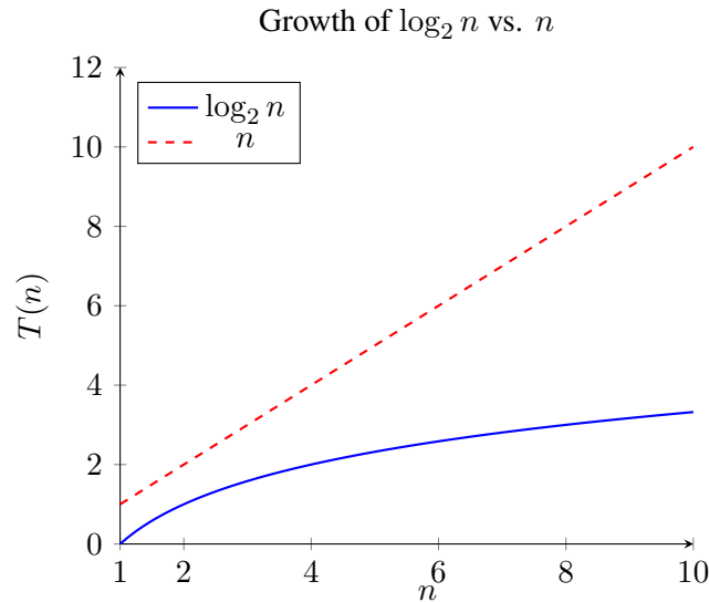
Figure 14.2: Graph comparing the growth rates of \log_2 n and n
