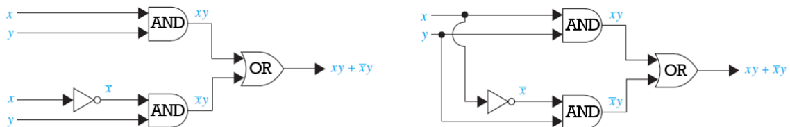
Figure 13.5: Two Equivalent Logic Gates. (Rosen, 2012).
