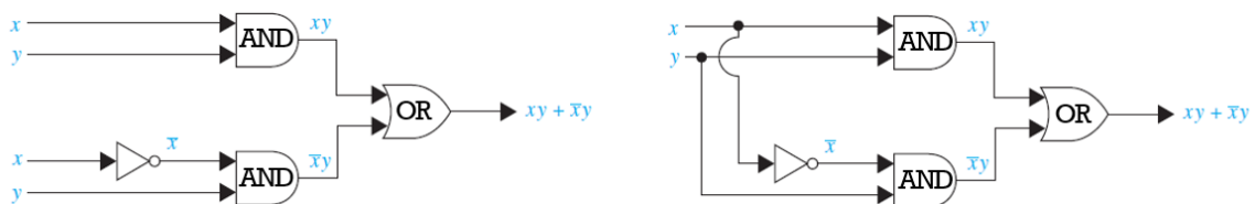
Figure 13.5: Two Equivalent Logic Gates. (Rosen, 2012).
