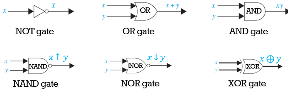
Figure 13.4: ANSI Symbols of Most Common Logic Gates. (Rosen, 2012).
