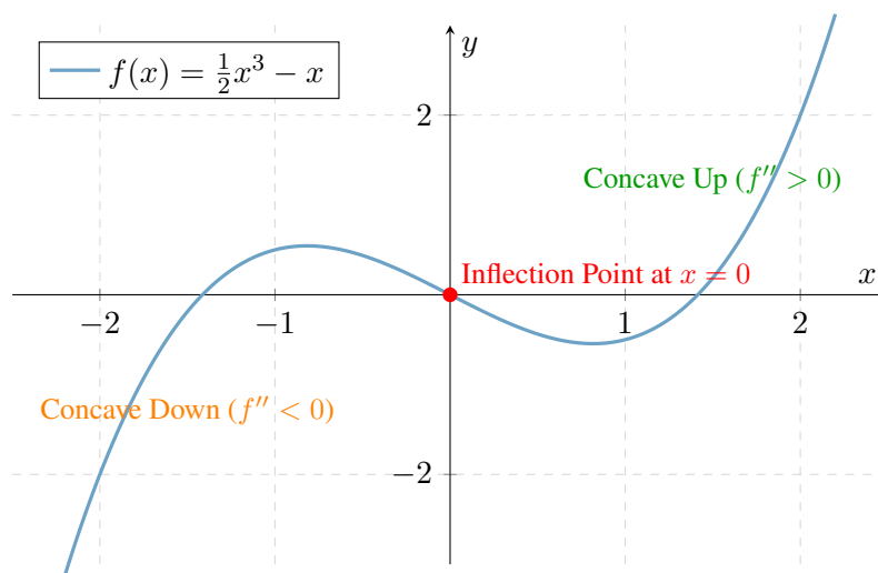
Figure 10.10: A function showing a region of concave down curvature, followed by a region of concave up curvature. The transition occurs at the inflection point.
