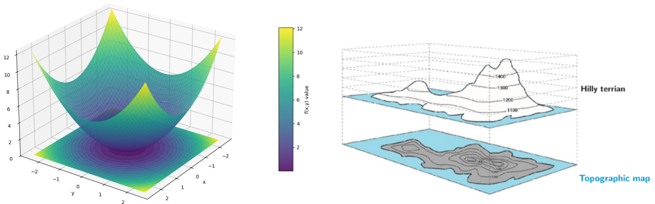
Figure 11.3: Contour Maps: (a) a 3D surface plot with contour lines projected onto the xy -plane, and (b) a topographic map showing level curves.
