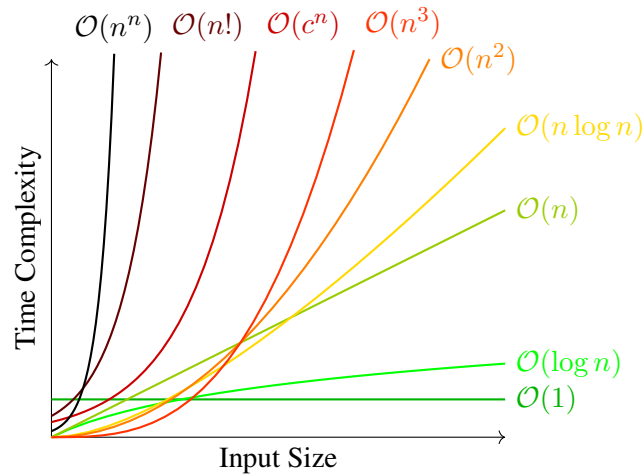
Figure 14.3: Conceptual illustration of time complexities
