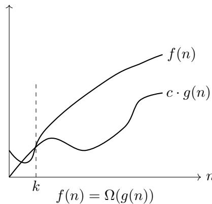
Figure 14.6: Illustration of \Omega -notation showing f(n) is asymptotically bounded below by c \cdot g(n) for large values of n .
