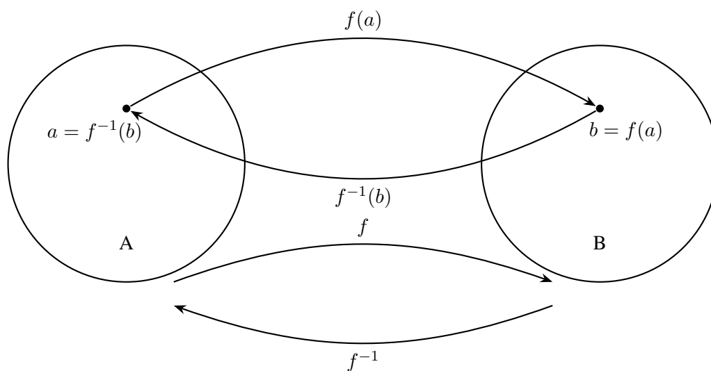
Figure A.2: The function f^{-1} is the inverse of function f .
