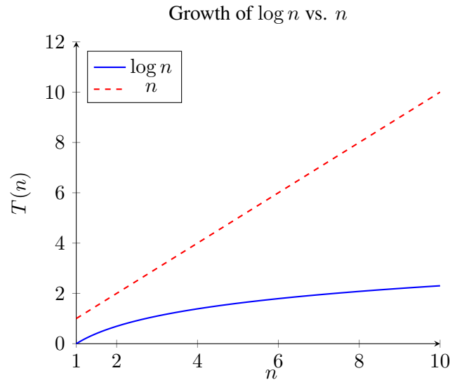
Figure 14.2: Graph comparing the growth rates of \log n and n
