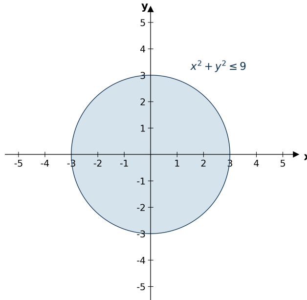
Figure 11.2: The domain of the function g(x, y) = \sqrt{9 - x^2 - y^2} is a closed disk of radius 3 .
