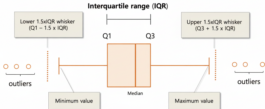
Figure 6.14: An example of a box plot, illustrating the median, quartiles, whiskers, and potential outliers.
