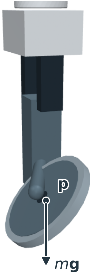
Figure 8: Reference apparatus of the real-robot validation, rendered in MuJoCo. (a) A steel disc is attached after bracket calibration. Its center of mass p and weight mg define the point and force references. The protocol uses eight mounting positions and masses of 0.5, 1.0, and 1.5 kg; a 1-kg disc of radius 60 mm is shown. (b) A force gauge presses at a marked dimple p . Two passive slide directions (double-headed arrows) allow lateral following while fixing the gauge axis in the world frame; the operator supplies the axial force f . The protocol uses eight marked points and approximately 10 and 20 N. Fixture geometry is schematic.
