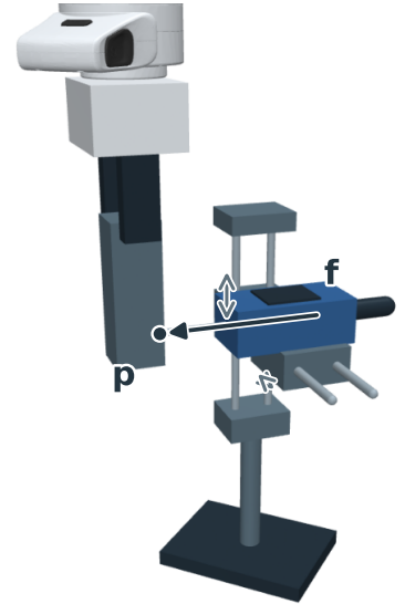
Figure 8: Reference apparatus of the real-robot validation, rendered in MuJoCo. (a) A steel disc is attached after bracket calibration. Its center of mass p and weight mg define the point and force references. The protocol uses eight mounting positions and masses of 0.5, 1.0, and 1.5 kg; a 1-kg disc of radius 60 mm is shown. (b) A force gauge presses at a marked dimple p . Two passive slide directions (double-headed arrows) allow lateral following while fixing the gauge axis in the world frame; the operator supplies the axial force f . The protocol uses eight marked points and approximately 10 and 20 N. Fixture geometry is schematic.
