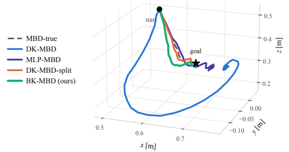
Fig. 2: Executed tool paths on one goal, one of the trials Table II counts. The five runs share the planner, the training seed and the random stream, so they differ in the rollout model alone.
