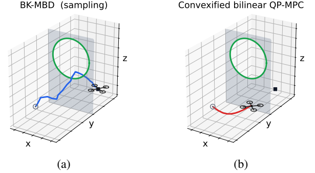
Fig. 3: Non-convex passage on the drone. The wall admits a single circular aperture. (a) BK-MBD threads the aperture and reaches the far-side goal, while (b) the convexified bilinear controller holds the near side.
