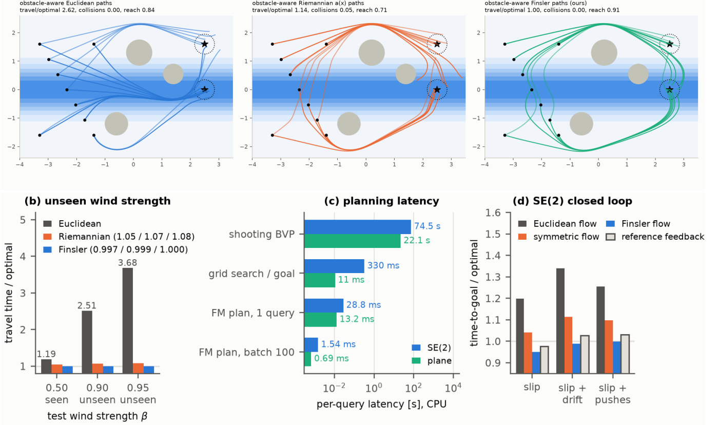
Fig. 4. (a) Plans with three obstacles in the head-wind channel; all planners are obstacle-aware, and the Finsler planner combines obstacle clearance with a downwind approach (reach 0.91, collisions 0, median ratio 0.999, worst 1.05). (b) One \beta -conditioned planner trained on \beta \in [0.30, 0.85] and tested at unseen wind strengths. (c) Per-query latency of the learned planner against the solvers that produced its training data. (d) SE(2) closed-loop execution under disturbances; all methods reach every goal, and the Finsler feedback field matches the reference value-function descent.
