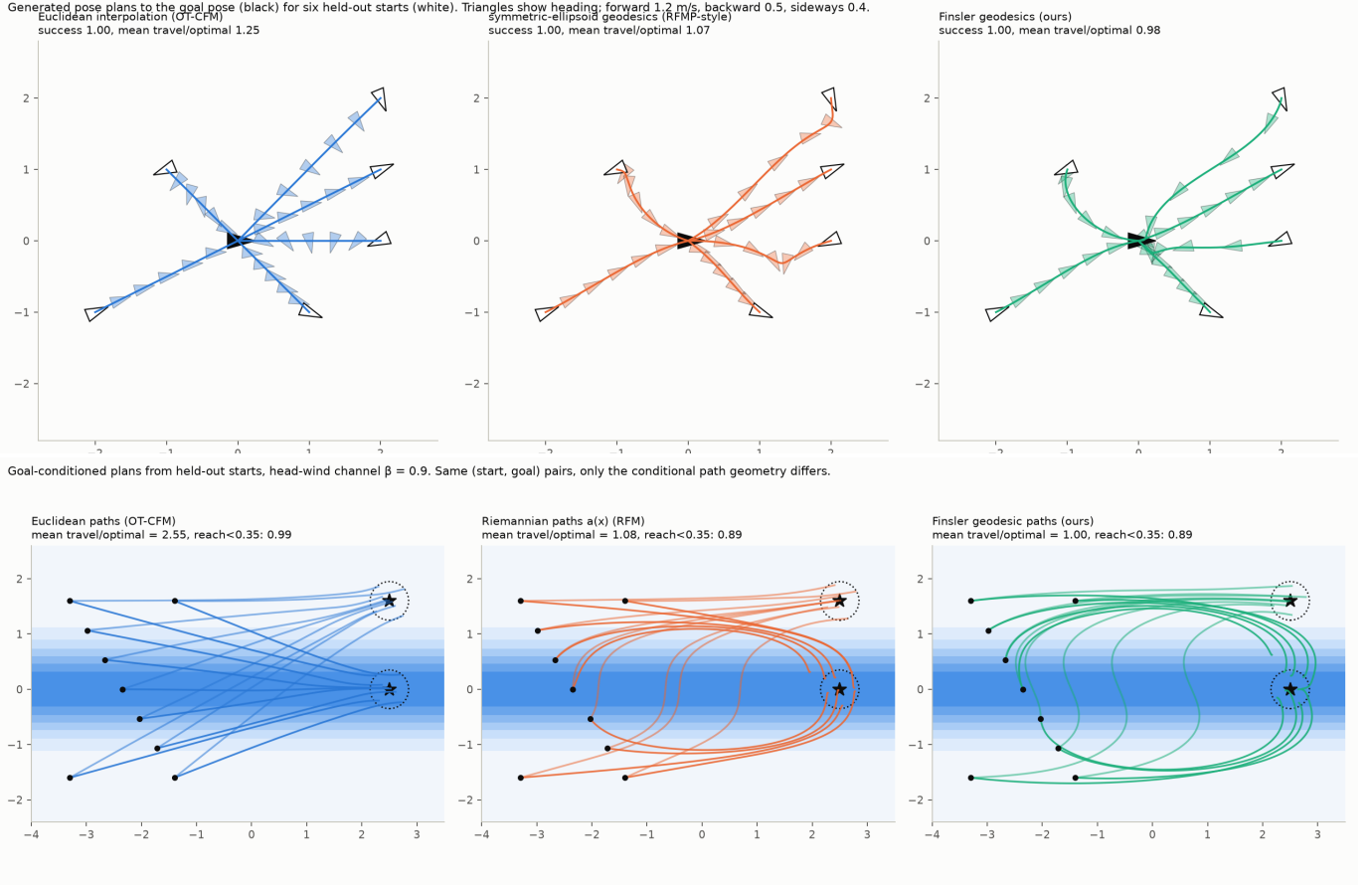
Fig. 3. Riemannian versus Finsler plans. Top: SE(2) plans to the origin pose from held-out start poses; Finsler plans turn towards the goal, walk forward and align the heading at the end, the symmetric planner backs up to goals behind the robot at the averaged fore-aft speed, and the Euclidean planner slides sideways. Bottom: plans in the head-wind channel ( \beta = 0.9 ) for the same start-goal queries; Euclidean paths cross the channel core at speed 0.1, Riemannian paths detour but enter the core goal from the upwind side, and Finsler paths detour widely and enter the core goal downwind, reproducing the structure of Zermelo-optimal paths. Time-to-goal over optimal, averaged over 98 queries: Euclidean 2.58, Riemannian 1.15, Finsler 1.06.
