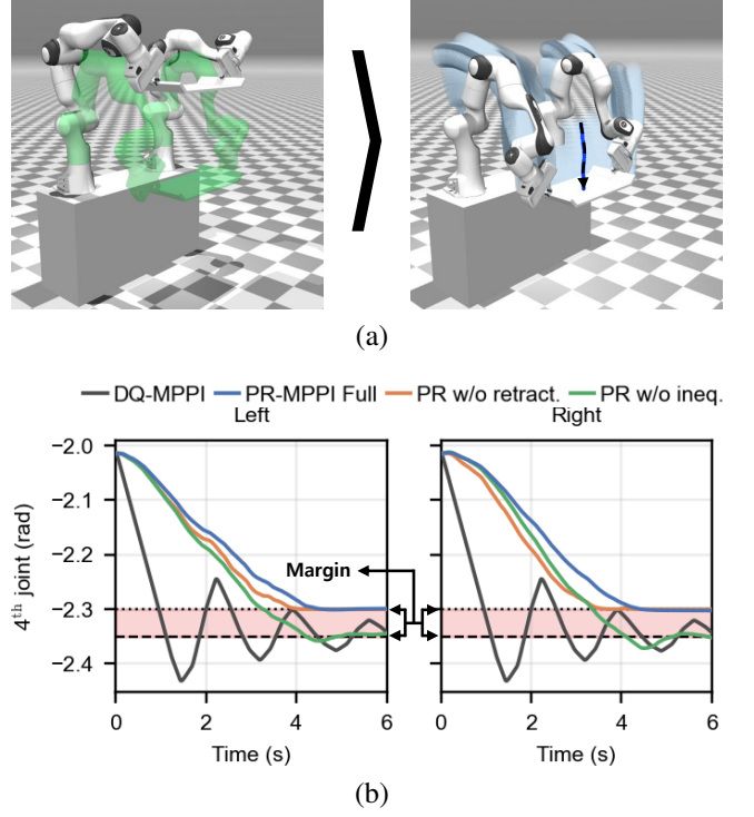
Fig. 2. Joint-limit stress test. (a) Dual-arm tray-lowering motion: the goal joint configuration in green and the trajectory executed by Full PR-MPPI in blue. (b) Measured fourth-joint trajectories of both arms for the four controllers. The dashed line is the artificial lower bound q_{4,\min} = -2.35 rad and the dotted line the shifted guard boundary at -2.30 rad; the shaded band between them is the 0.05 rad CBF margin.
