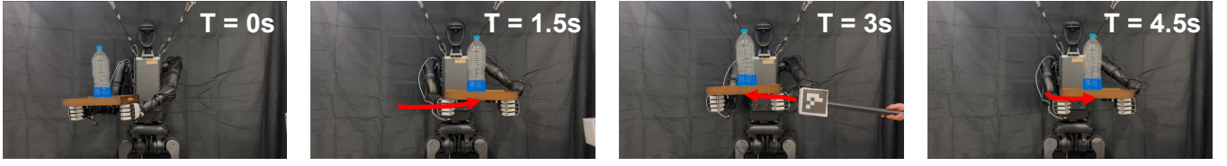
Fig. 4. Hardware demonstration on the Unitree H1-2. The two arms hold a tray carrying a payload under the closed-chain grasp while a hand-held obstacle is moved toward it; each frame is labelled with the elapsed time.
