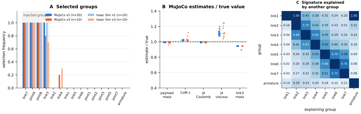
Figure 4: Selection stability and group separation. (A) Selection frequency of each group over 20 (MuJoCo, noise \times 1 ), 10 (MuJoCo, \times 3 ) and 10 (Isaac Sim, \times 1 and \times 3 ) sensor-noise realisations. (B) MuJoCo estimates normalised by the true value; the link-3 mass is a structurally unidentified direction. (C) Fraction of a group's standardised torque signature explained by another group's column space on the identification rows.
