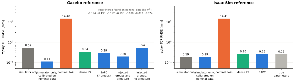
Figure 5: Cross-simulator decomposition of the replay TCP RMSE. Left, Gazebo: calibrating on nominal Gazebo data alone discovers the missing rotor inertia of all seven joints and reduces the simulator-only discrepancy from 0.52 to 0.11 mm; removing the armature from the calibrated twin raises the error above the simulator-only level. Right, Isaac Sim: the rotor inertia is preserved, calibration on nominal data returns no correction, and the calibrated twins reach the matched-parameter twin.
