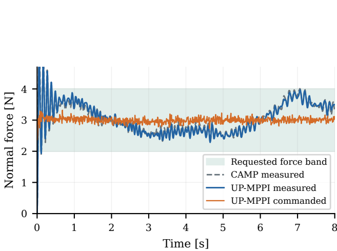
(a) Commanded and measured reaction, zero offset
