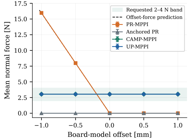
(b) Contact force versus board-model offset
